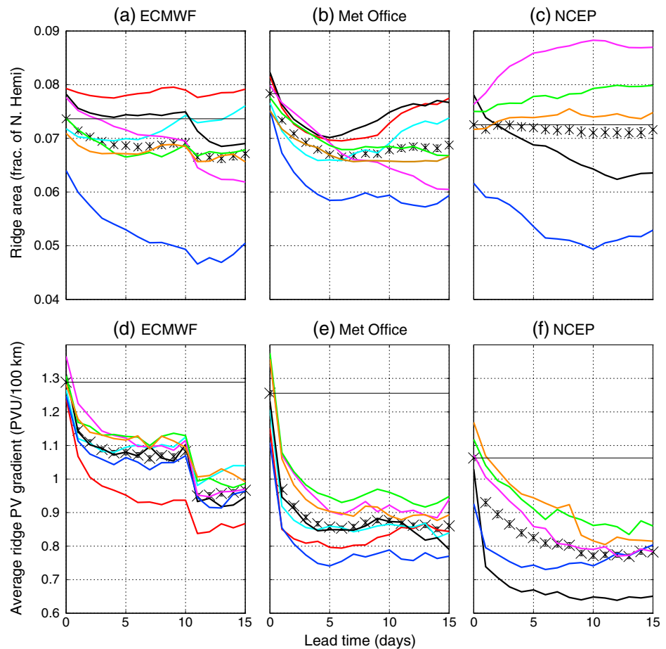
Figure 5. (a–c) Average ridge area and (d–f) the isentropic PV gradient flanking ridges as a function of forecast lead time for ECMWF, Met Office, and NCEP. Black markers with error bars (standard errors) are averages over all winter seasons with horizontal lines extending across all lead times from the analysis values. Colored lines are averages for the individual seasons where red is 2006/2007, cyan is 2007/2008, black is 2008/2009, blue is 2009/2010, magenta is 2010/2011, green is 2011/2012, and orange is 2012/2013. Note (as an example) that a fraction of the Northern Hemisphere of 0.05 is equivalent to an area of 1.275 \times 10^7 \text{ km}^2 .
