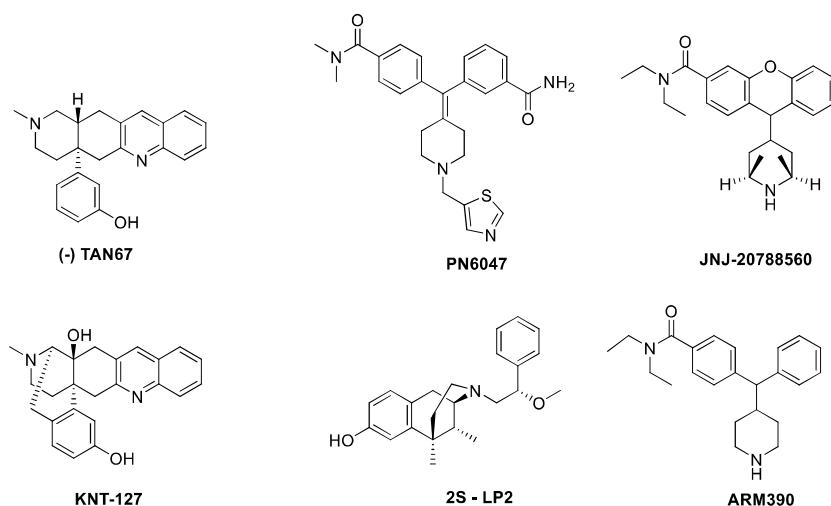
Figure 4. Structures of DOR biased ligands reported having different levels of \beta -arrestin 2 recruitment.
