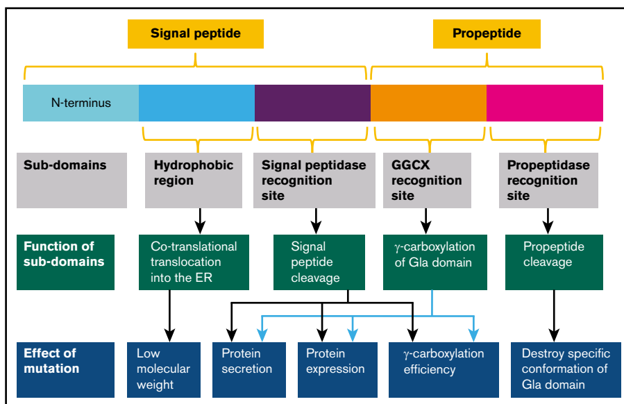
Figure 6. The effect of mutations on functional subdomains of FIX signal peptide and propeptide. The signal peptide consists of 2 subdomains: the hydrophobic region and the signal peptidase recognition site. The hydrophobic region is recognized by signal recognition particles that assist in cotranslational translocation of FIX into the ER; mutations in the region lead to a lower MW. Mutations in the signal peptidase recognition site interfere with protein secretion, expression, and \gamma -carboxylation efficiency by preventing signal peptide cleavage. The propeptide region includes 2 subdomains: the GGCX recognition site and the propeptidase recognition site. Mutations in the GGCX recognition site affect protein secretion, protein expression, or \gamma -carboxylation efficiency. Mutations in the propeptidase recognition site lead to unremoved propeptide and destroy the specific conformation of the Gla domain.
