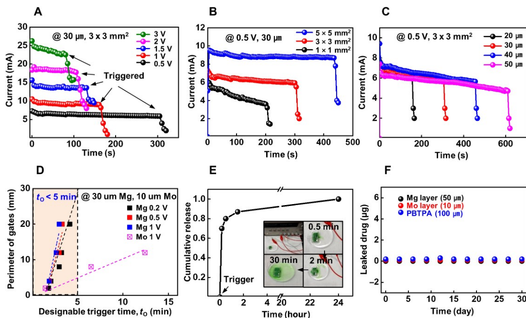
Fig. 3. Trigger and release behaviors of bioresorbable drug delivery vehicles with electrochemical control. (A) Dependence of the trigger time on applied potential at fixed Mg gate size (30 \mu m thickness, 3 mm by 3 mm area). (B) Effect of the exposed area of the gate on trigger time at a fixed applied potential (0.5 V) and gate thickness (30 \mu m). (C) Dependence of trigger time on thickness of the gate, for a fixed applied potential (0.5 V) and gate area (3 mm by 3 mm). (D) Comparison of the trigger time of Mg (30 \mu m at 0.2, 0.5, and 1 V) and Mo (10 \mu m at 1 V) gates for various perimeters of the gates. (E) Kinetics of the release of doxorubicin after triggering to open an area of 2 mm by 2 mm in the Mg gates. (F) Leakage of drug (doxorubicin) through the layers of material used for the reservoir and the gates [black, Mg (50 \mu m thick); red, Mo (10 \mu m thick); and blue, PBTPA 1:4:7 (100 \mu m thick)] during immersion in PBS at body temperature (37°C). Photo credit: Jahyun Koo, Korea University.
