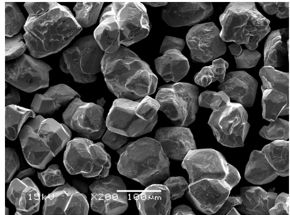
Fig. 3. Tungsten powder was imaged using a JEOL 6060LV general purpose scanning electron microscope. The powder is sold as Technon Tungsten Powder 100 mesh, with 90% of the particles ranging in size between 25 and 150 \mu\text{m} . This wide distribution allows for higher packing density within each block.
