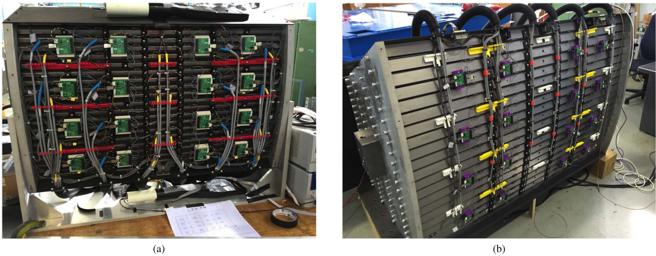
Fig. 10. Fully assembled (a) inner and (b) outer HCals. Each section has 20 steel absorber plates stacked together and 80 scintillating tiles are inserted between them. SiPMs read out from five tiles are ganged together like a tower. This results in a total of 16 towers equipped with SiPM sensors, preamplifiers, and cables carrying the differential output of the preamplifiers to the digitizer system.
