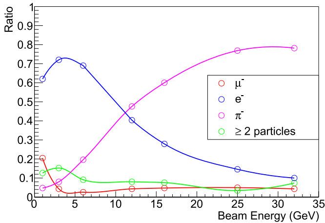
Fig. 14. Relative abundance of particle species present in the FTBF negatively charged beam as a function of beam energy [25].
