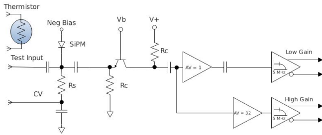
Fig. 11. Schematic for the inner HCal preamplifier. For the EMCAL and the outer HCal preamplifier, the high-gain channel is \times 16 the normal (low-gain) channel. In addition, the EMCAL design included a programmable selection of either the high-gain or normal-gain channel as output to the digitizers.
