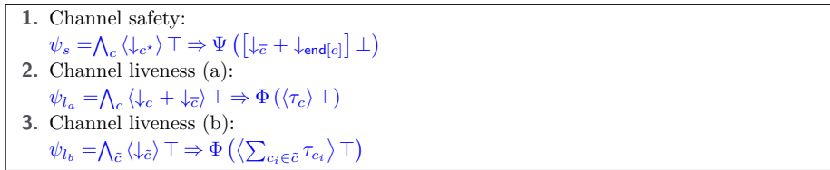
■ Figure 16 Modal \mu -calculus properties for channels.
