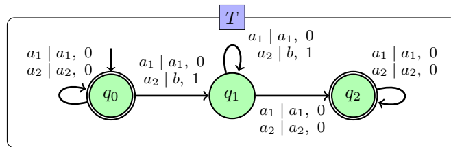
■ Figure 1 A weighted-transducer over \Sigma = \{a_1, a_2, b\} .
