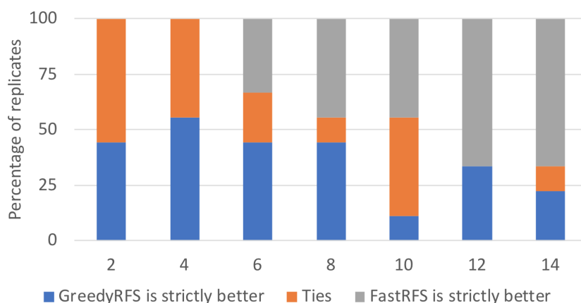
■ Figure 5 Results for Experiment 2: The percentage of datasets ( y -axis) that each method (FastRFS and GreedyRFS) ties with or is strictly better than the other in terms of RFS criterion score is shown for varying numbers of source trees ( x -axis), based on nine replicate supertree 500-leaf 20% scaffold datasets (from [39]).
