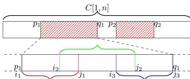
■ Figure 2 \mathcal{T} as a union of disjoint subsets.
