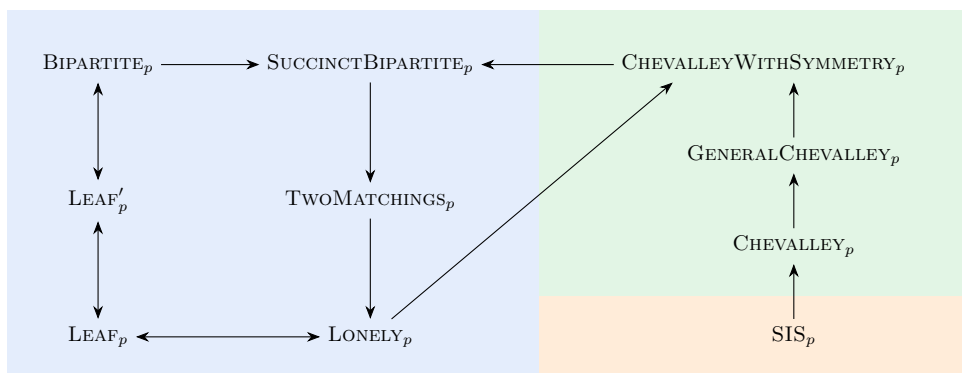
■ Figure 2 Total search problems studied in this work. An arrow A \rightarrow B denotes a reduction A \leq B that we establish. Problems in the blue region are non-natural problems, which are all complete for \text{PPA}_p . Problems in the green region are natural problems of which \text{CHEVALLEYWITHSYMMETRY}_p is the one we show to be \text{PPA}_p -complete. The problem in the orange region is a cryptographically relevant problem.
