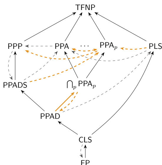
■ Figure 1 The landscape of TFNP subclasses. A solid arrow M_1 \rightarrow M_2 denotes M_1 \subseteq M_2 , and a dashed arrow M_1 \dashrightarrow M_2 denotes an oracle separation: M_1^\mathcal{O} \not\subseteq M_2^\mathcal{O} relative to some oracle \mathcal{O} . The relationships involving PPA_p are highlighted in yellow. See Section 7 for details.
