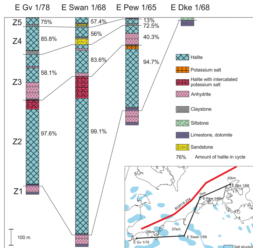
Figure 3. Correlation of Zechstein cyclothem along the northeast North German Basin margin. Z1 = Werra; Z2 = Stassfurt; Z3 = Leine; Z4 = Aller; Z5 = Ohre. Well information compiled after Hoth et al. (1993). Inset: salt structures after Reinhold et al. (2008). Numbers represent approximate distance from the well to similar position regarding salt distribution on the profile BGR16-254 (see also Figure 1 for location).
