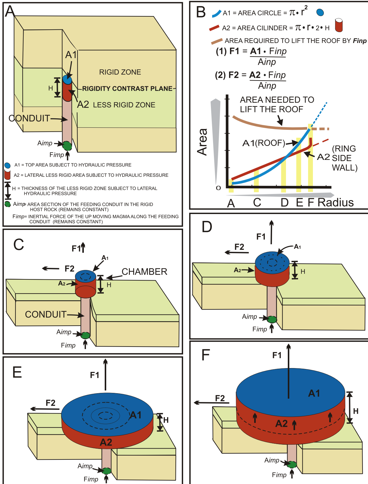
Figure 2. Schematic model for magma chamber growth using Pascal's hydraulic principle in lateral and vertical hydraulic jack geometries. (A) Ascending magma in a conduit intrudes a less rigid zone (portion H) is prevented from continuing when reaching a more rigid zone that forces a lateral expansion and widening of the conduit and development of an incipient chamber. (B) Area/Radius growth diagram. For simplicity, the magma chamber growth is modelled using the expansion of a cylinder in the less rigid zone. The roof area is circular and shows an exponential growth curve with the square of the radius. The area of the lateral ring wall is that of a cylinder and increases linearly with radius. Since hydraulic force multiplication depends on the relationship between areas, this Area/Radius diagram predicts that deformation begins as lateral growth followed later by vertical growth. The brown line represents schematically the area that the sill roof should reach so that the hydraulic jack output force is capable of breaking the tensile/compressive strength that supports the roof to the side wall and lift the roof; thus, as distance between the side walls increases the tensile strength is the main force keeping the roof integrity. In
