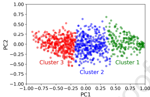
Figure 2. Principal Components from PCA. Colors represent three different data clusters obtained by K-Means algorithm. Dots color intensity represents outcome frequency
