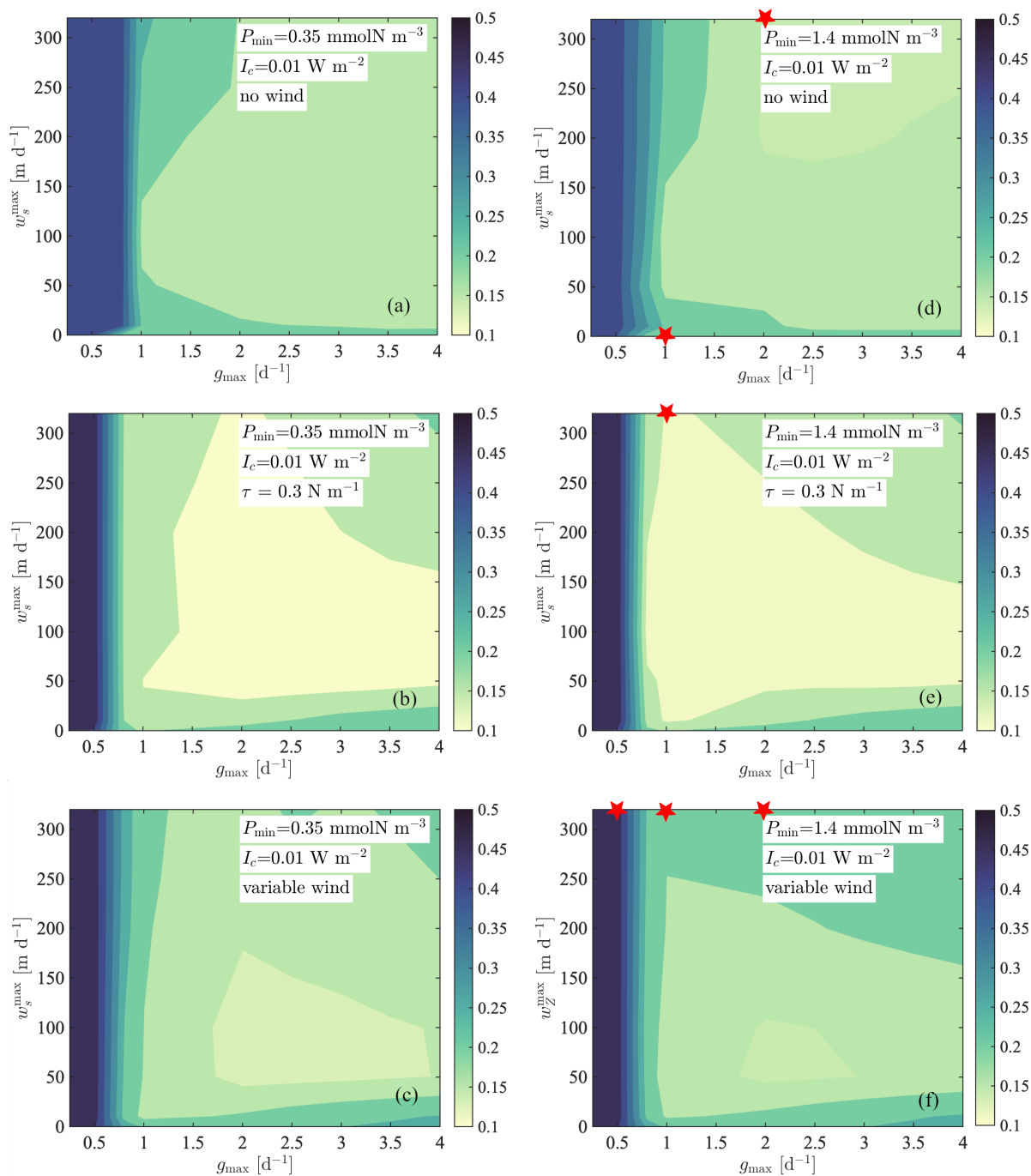
Figure 8. Carbon export indicator ( \Phi ) representing the last 20 meters of the water column for two minimum phytoplankton concentrations 0.35 and 1.4 \text{mmolN m}^{-3} (left and right columns, respectively) and different wind forcings: no wind stress ( a and d ), constant wind stress 0.3 \text{N m}^{-1} ( b and e ) and variable wind stress ( c and f ). The critical irradiance is the same and equal to 0.01 \text{W m}^{-2} for all panels. Red stars refer to the examples in Fig. 4.
