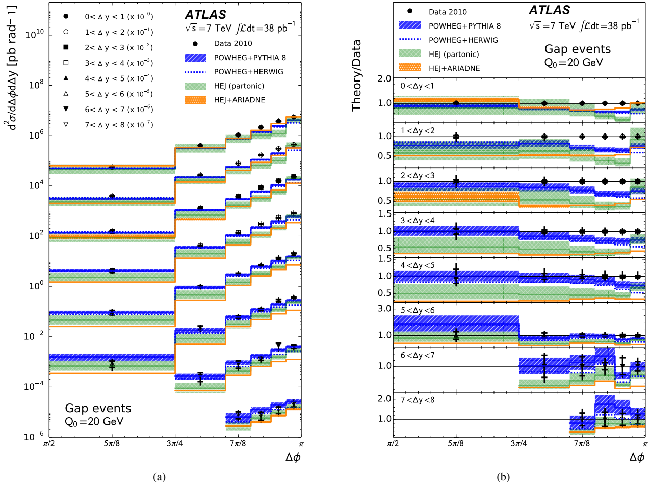
Fig. 8: The measured double-differential cross sections as a function of \Delta\phi for eight slices in \Delta y , for gap events. The veto scale is Q_0 = 20 \text{ GeV} . For comparison, the HEJ, HEJ+ARIADNE, POWHEG+PYTHIA 8 and POWHEG+HERWIG predictions are presented in the same way as Fig. 3. In (a) the absolute comparison is shown, while in (b) the ratios of the predictions to the data are shown.
