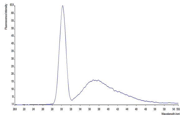
Figure 2. Excitation and emission spectra of menbutone (1.2 \mu\text{g/mL} ).
