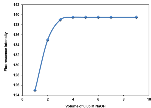
Figure 5. Effect of volume of NaOH on the fluorescence intensity of menbutone (1.0 \mu\text{g/mL} ).
