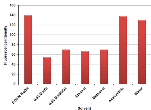
Figure 4. Effect of different solvents on the fluorescence intensity of menbutone (1.0 \mu\text{g/mL} ).
