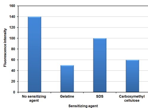
Figure 3. Effect of different sensitizing agents on fluorescence intensity of menbutone (1.0 \mu\text{g/mL} ).
