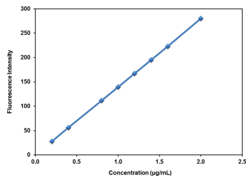
Figure 6. Calibration curve of the fluorescence intensity ( \lambda_{em} = 378 nm, \lambda_{ex} = 300 nm) to concentrations of menbutone.
