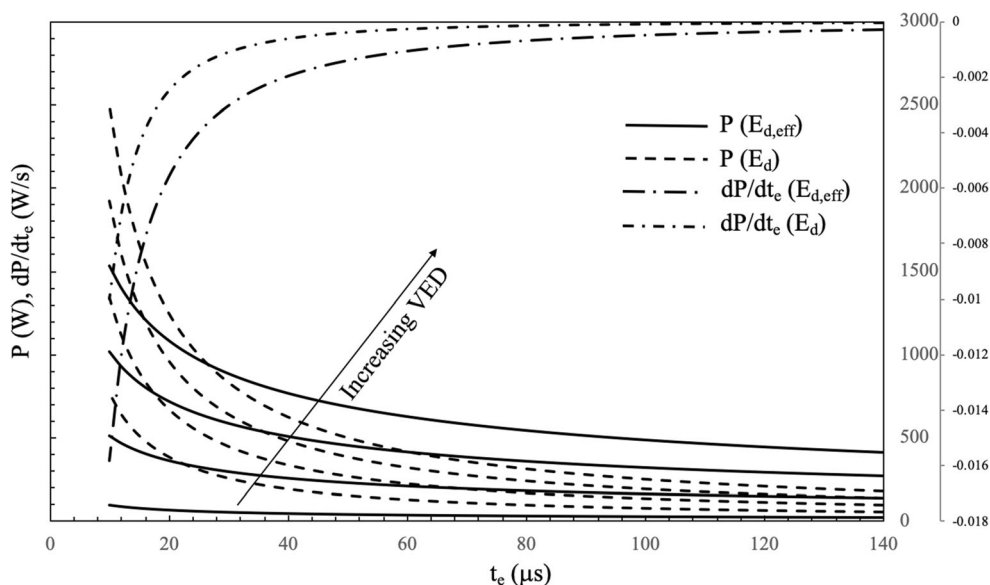
Fig. 6 Iso-energy density curves and their derivatives
