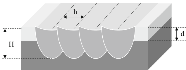
Fig. 5 Schematic of volumes effectively affected by the heat source (with H = heated depth)
