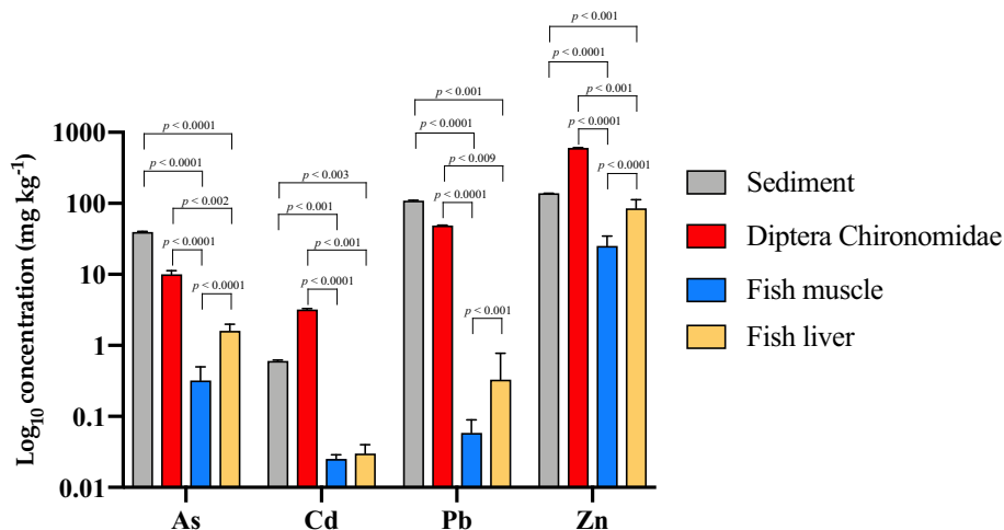
Fig. 2. Trace element concentration (Log 10 ) detected in sediment, Diptera Chironomidae, and fish muscle and liver samples. Results of post-hoc Conover Iman test are also reported to indicate significant differences between matrices.
