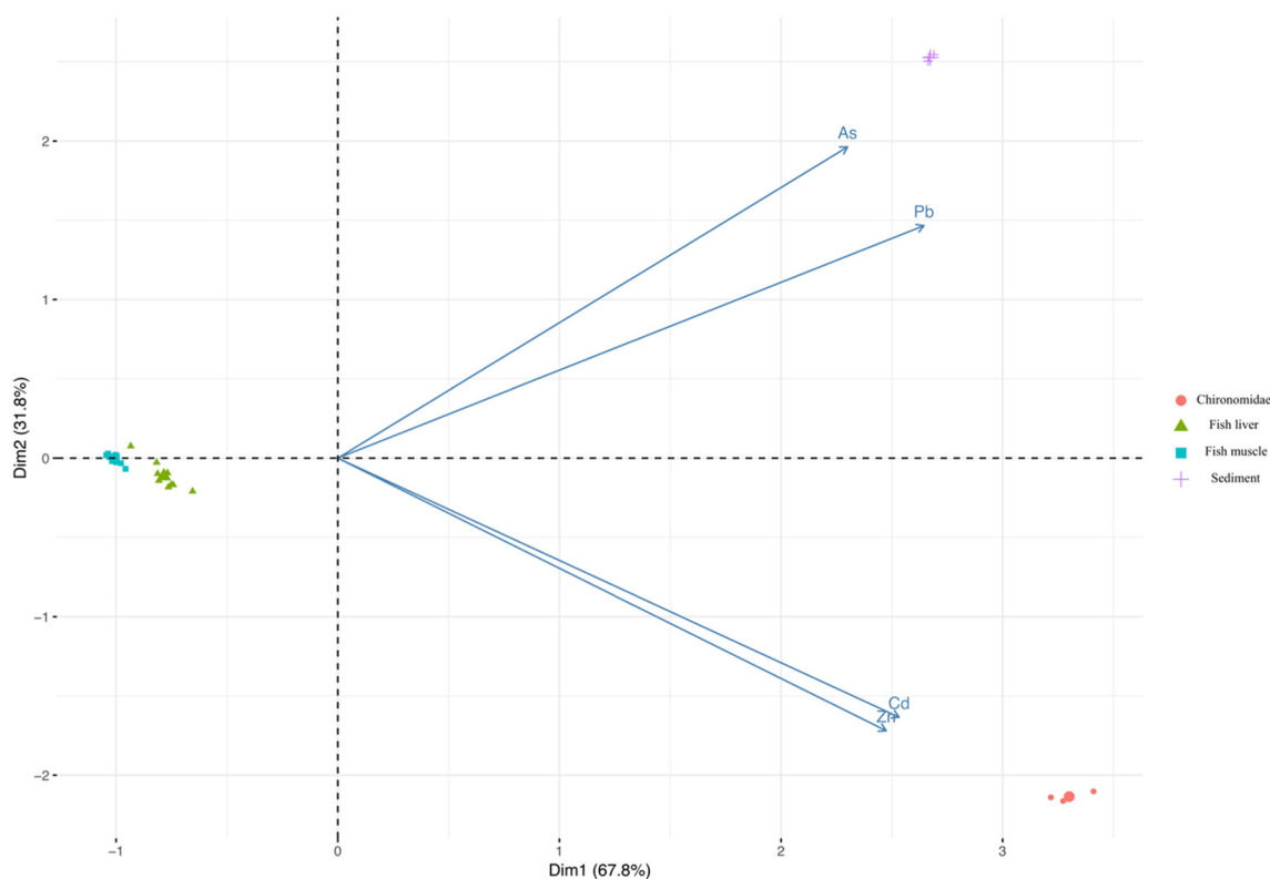
Fig. 3. Biplot of score and loadings from principal component analysis. The scores for the matrix (sediment, Diptera Chironomidae, fish liver and fish muscle) are denoted by a color and a symbol (largest symbol = average value).
