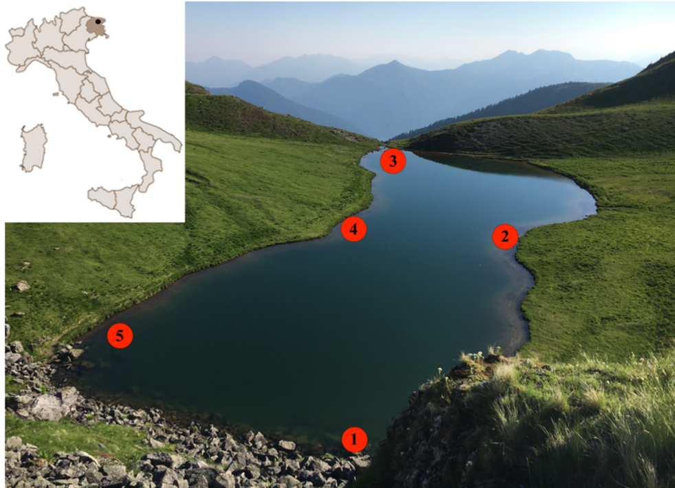
Fig. 1. Dimon Lake in Friuli Venezia-Giulia (northeast Italy) and sampling sites (1–5; red circles) for sediment and macrobenthic invertebrates. (For interpretation of the references to color in this figure legend, the reader is referred to the web version of this article.)
