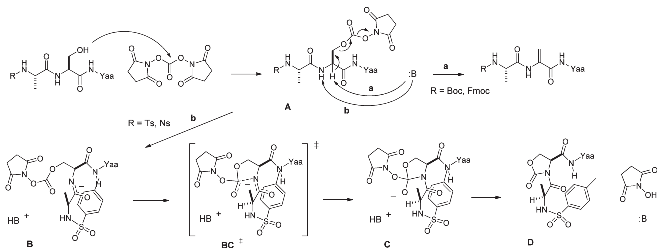
Scheme 3 Plausible reaction pathways for the elimination of carbamate-peptides (pathway a ) and alternatives for the cyclization of arylsulfonfyl peptides (pathway b ).
