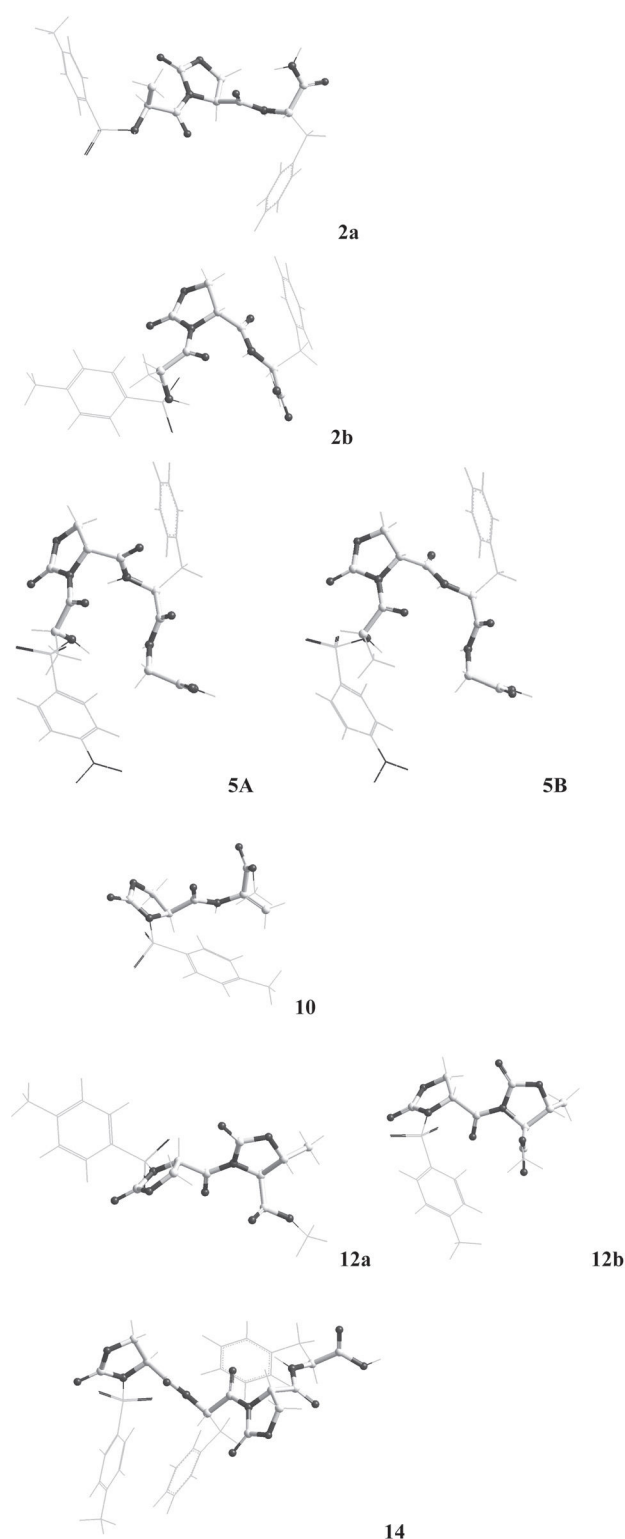
Fig. 2 Representative low-energy structures of 2a , 2b , 5 (A, B) , 10 , 12a , 12b , 14 consistent with ROESY analysis, calculated by restrained MD in a 30 × 30 × 30 box of standard TIP3P water molecules. Backbones and Oxd are rendered in balls and cylinders, the rest in sticks.
