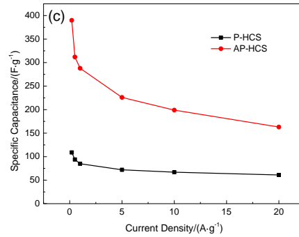
图 6 P-HCS 和 AP-HCS 在 1mol/L H 2 SO 4 电解液中的 CV 曲线 (a)、GCD 曲线 (b) 和不同电流密度下的比电容 (c) Fig.6 CV curves (a), GCD curves (b) and specific capacitances calculated from GCD at various current densities (c) of P-HCS and AP-HCS in 1M H 2 SO 4
