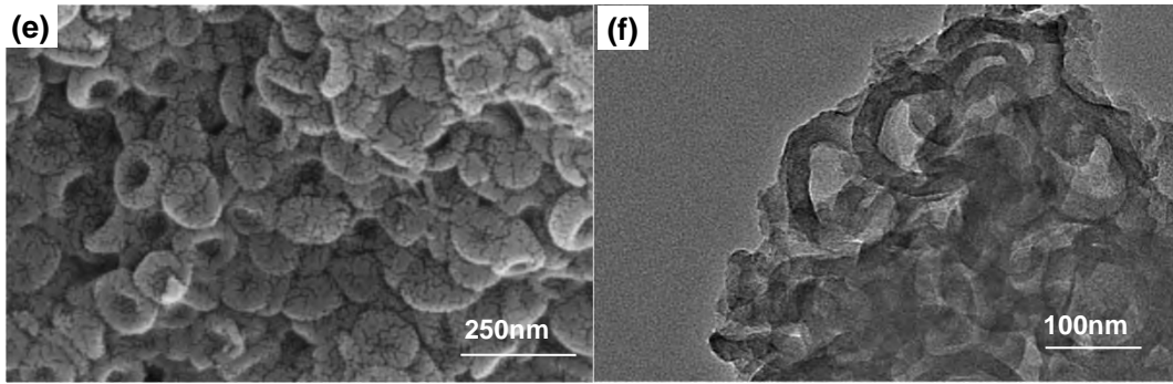
图3 SEM图和TEM图: HPS (a) (b); P-HCS (c) (d); AP-HCS (e) (f) Fig.3 SEM and TEM images : HPS (a) (b); P-HCS (c) (d) and AP-HCS (e) (f)
