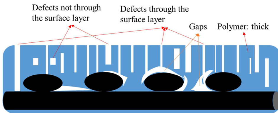
(a): many tiny pores in the surface polymer layer of E-CFRP
