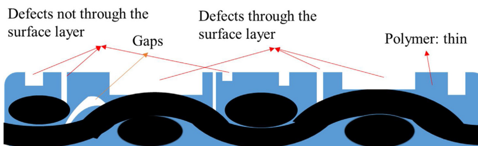
(b): few large pores in the surface polymer layer of T-CFRP
