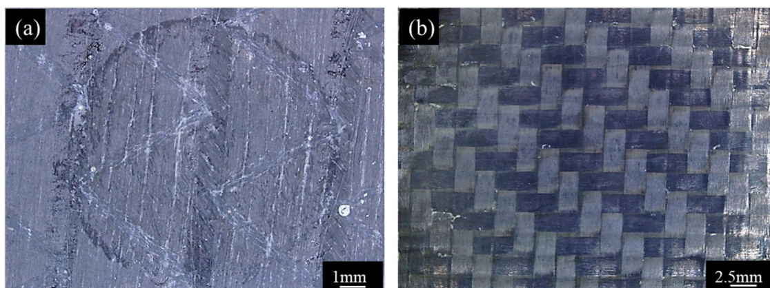
Fig. 11 – Morphologies of exposed areas of (a) E-CFRP (not ground) and (b) T-CFRP (not ground) after 4 weeks of testing.
