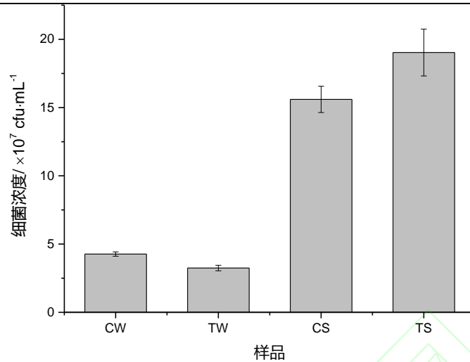
图3 功能化石墨烯对海水和海洋沉积物样品中细菌细胞浓度的影响 Fig. 3 Effect of functionalized graphene on concentration of bacterial cells in seawater and marine sediment
