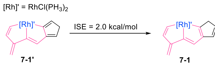
Figure S14. ISE evaluation of model complex 7-1' , related to Scheme 4.
