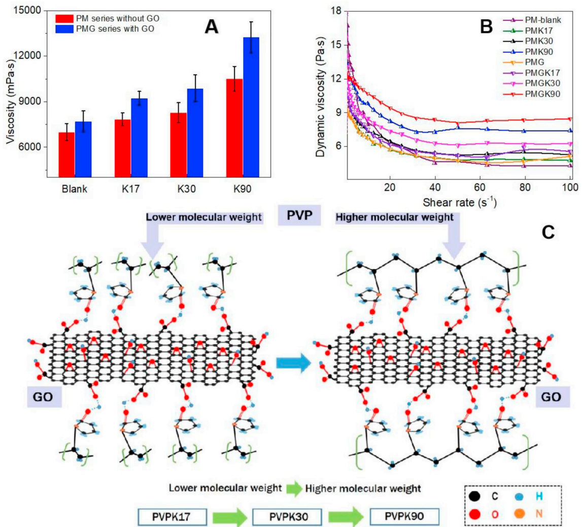
Fig. 1 Viscosity of casting solutions (A), the dynamic viscosity versus shear rate (B) and the interactions between GO and PVP with different MWs (C).
