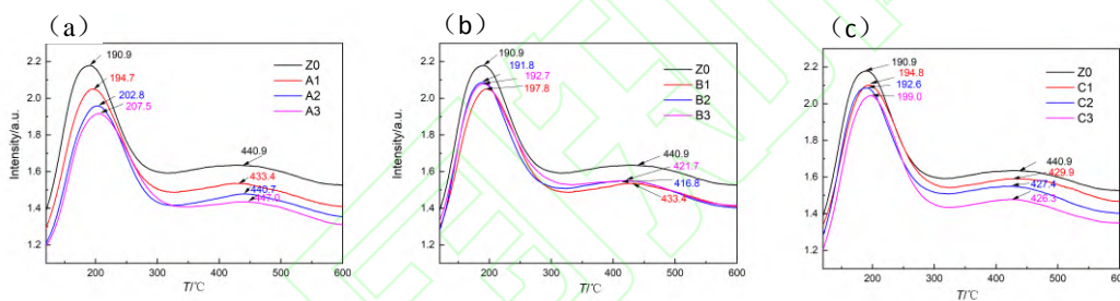
图 2 不同水蒸气条件改性处理后 H-FER 分子筛 \text{NH}_3 -TPD 图谱 Fig.2 \text{NH}_3 -TPD diagram of H-FER zeolites modified by steam treatment conditions
