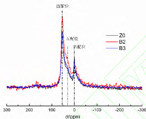
图 5 不同条件水蒸气处理前后 H-FER 分子筛的 ^{27}\text{Al} MAS NMR 图谱 Fig.5 ^{27}\text{Al} MAS NMR spectrum of H-FER zeolites modified by different steam treatment conditions
