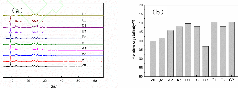
图 1 不同条件水蒸气处理后 H-FER 分子筛 XRD 谱图和相对结晶度对比图 Fig. 1 XRD patterns and relative crystallinity of H-FER zeolites modified under different water vapor treatment conditions
