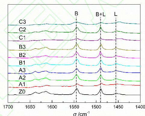
图 3 不同水蒸气条件改性处理后 H-FER 分子筛 Py-IR 图谱 Fig.3 Py-IR Infrared spectrum of H-FER zeolites modified by different steam treatment conditions
