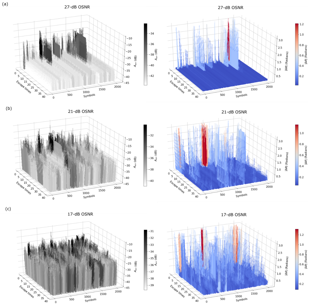
Fig. 14: A_{err} (left) and absolute phase error |\Delta\theta| (right) for all the symbols after each escape with an OSNR of (a) 27 dB, (b) 21 dB and (c) 17 dB.
