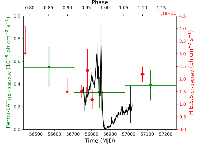
Fig. 4. Phase-binned H.E.S.S. flux above 190 GeV as red points. The phase errors in the H.E.S.S. light-curve points refer to the re-grouped data given in Tab. 1. Fermi –LAT \gamma -ray flux points from Balbo & Walter (2017) and Swift X-ray data from Corcoran et al. (2017) are shown as green triangles and as black line, respectively. Flux errors are all 1\sigma while upper limits are 95% confidence level. The X-ray data has been scaled to arbitrary units for better comparison to the \gamma -ray data.
