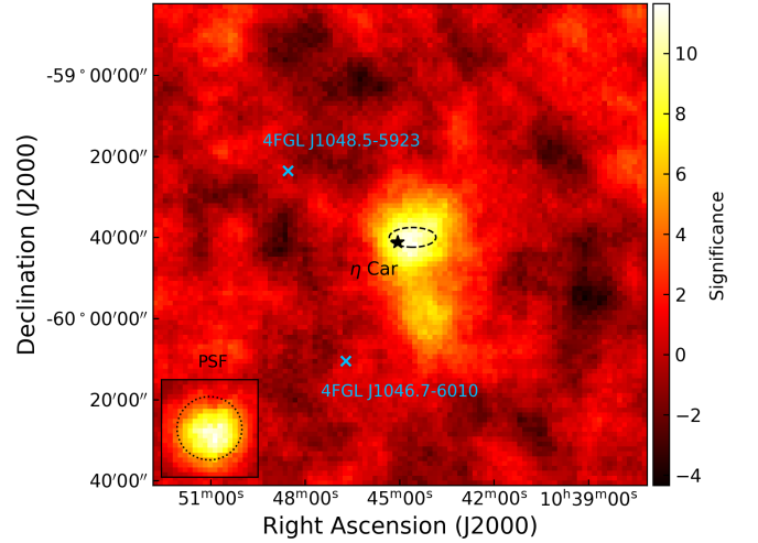
Fig. 2. Significance map as obtained in the CT5 mono analysis, for the combined DS-I ( 0.78 < p < 0.96 ) and DS-II ( 1.09 < p < 1.10 ) using an oversampling radius of 0.1^\circ . The position of \eta Car is denoted with a black star and the long-dashed ellipse refers to the uncertainty in the positional fit as described in the main text. The positions of the nearby Fermi -LAT sources 4FGL J1048.5–5923 and 4FGL J1046.7–6010 are shown with blue crosses (The Fermi -LAT collaboration 2019). The inlay shows the point spread function (PSF) as obtained using run-wise simulations (RWS) in colour, while the overlaid dotted circle indicates the PSF using classical simulations.
