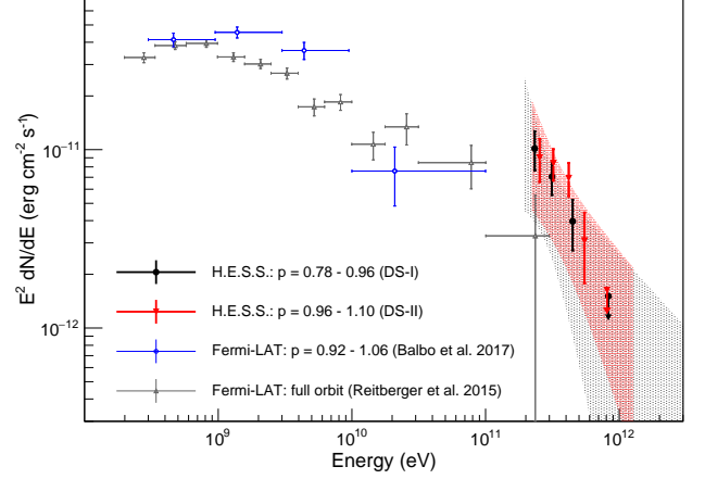
Fig. 3. Spectral energy distribution of \eta Car for DS-I (black) and DS-II (red). H.E.S.S. points show 1\sigma statistical errors. The shaded regions indicate the combined statistical and systematic errors (as given in the main text and Tab. 3). Fermi –LAT spectra from Reitberger et al. (2015) for the full orbit (grey) and for the last periastron passage from Balbo & Walter (2017) (blue) are also shown.
