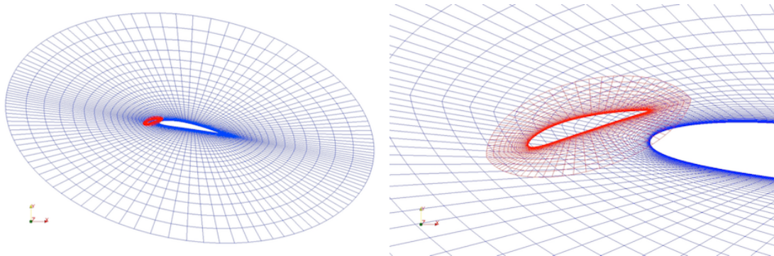
Figure 3: Grid(Over view) and Zoomed to around the leading edge
