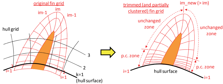
Figure 1: Trimming and partial clustering ( a fin attached to a hull): left:original, right: applied
