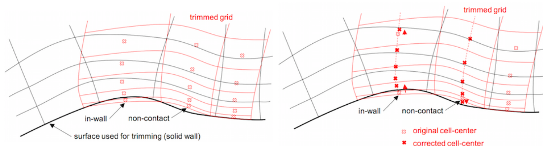
Figure 9: trim correction
