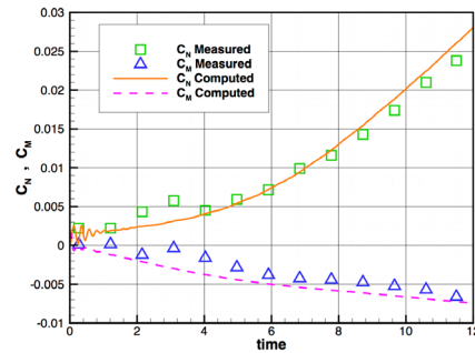
Figure 13: Normal force ( C_N ) and pitch moment ( C_M )
