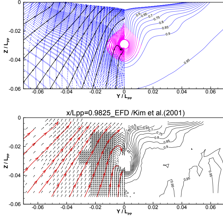
Figure 11: Cross flow vectors and streamlines(left) and axial velocity contours ( \Delta U = 0.05 )(right) at x/L_{PP} = 0.9825 . Top: Computed results, Bottom: Measured data
