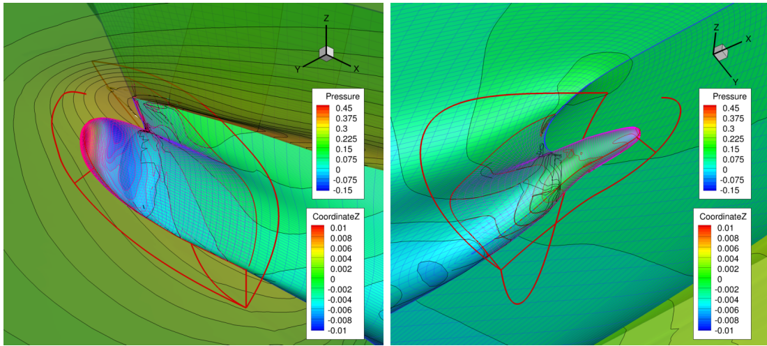
Figure 10: Schematic view of bow(left) and stern(right). Pressure distribution on the hull surfaces and wave elevation ( \Delta z = 0.0005 ) are also shown.
