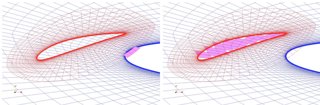
Figure 4: left: in-wall cells of the slat grid, right: in-wall cells of the wing grid
