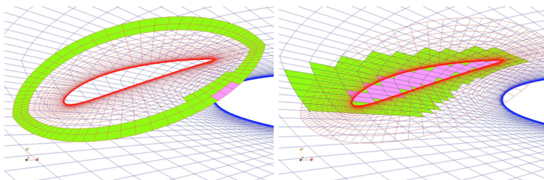
Figure 5: left: receptor_m cells of the slat grid, right: receptor_m cells of the wing grid)
