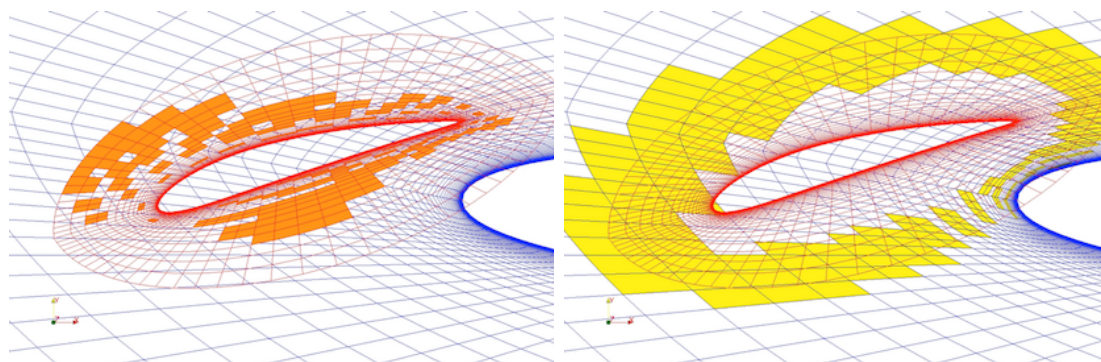
Figure 7: left: donor_m cells of the slat grid, right: donor_m cells of the wing grid
