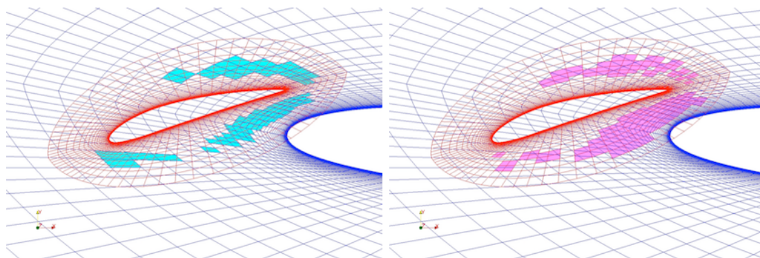
Figure 8: left: receptor_o of the wing grid right: donor_o of the slat grid
