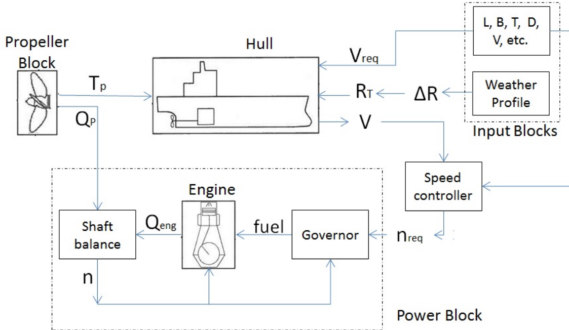
Figure 1: Overall ship simulator implementation in MATLAB/Simulink environment
