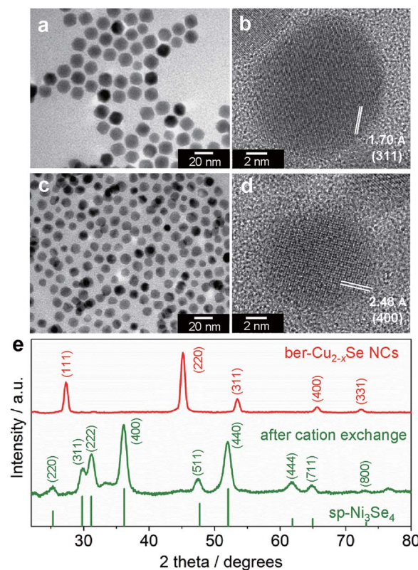
Fig. 1 (a and c) TEM and (b and d) HRTEM images of (a and b) ber-Cu 2–x Se NCs and (c and d) sp-Ni 3 Se 4 NCs. (e) XRD patterns of ber-Cu 2–x Se NCs and sp-Ni 3 Se 4 NCs. The reference XRD pattern shows sp-Ni 3 Se 4 (JCPDS 18-0889).
