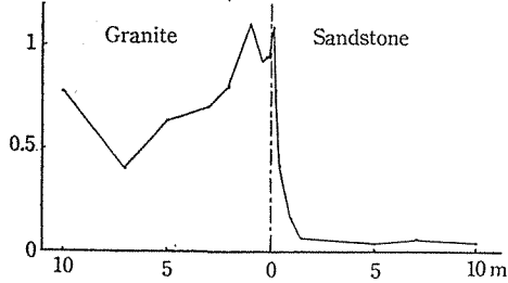
Fig. 6. Radioactive profiles. (Matsuyama)
