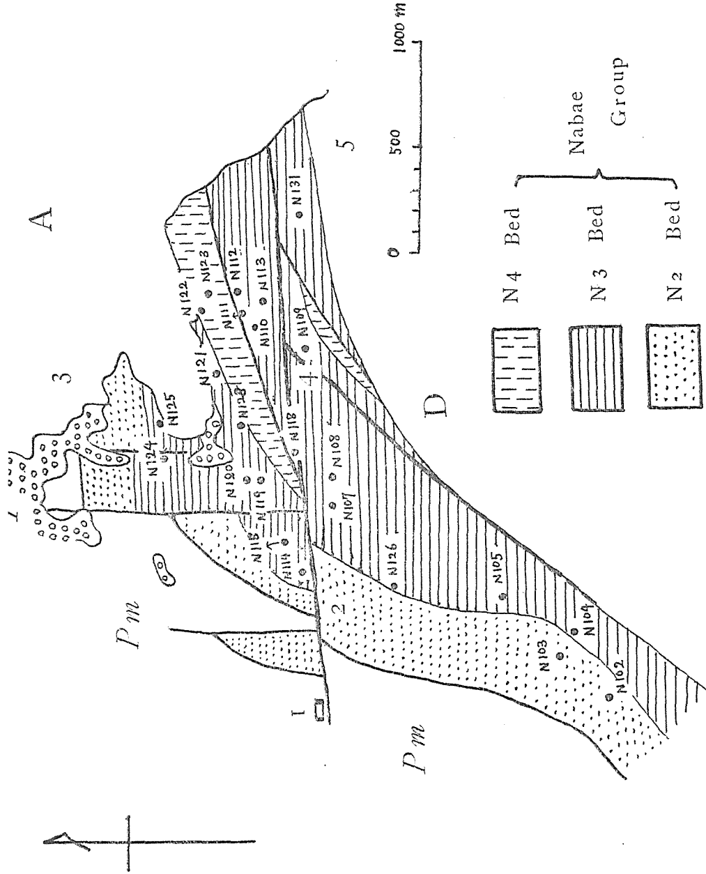
Fig. 2. Fossil Localities in Matsunodera Area.
