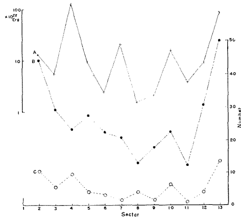
Fig. 4. Zonal variation along the arc of both frequency and released energy for earthquakes belonging to each sector.
