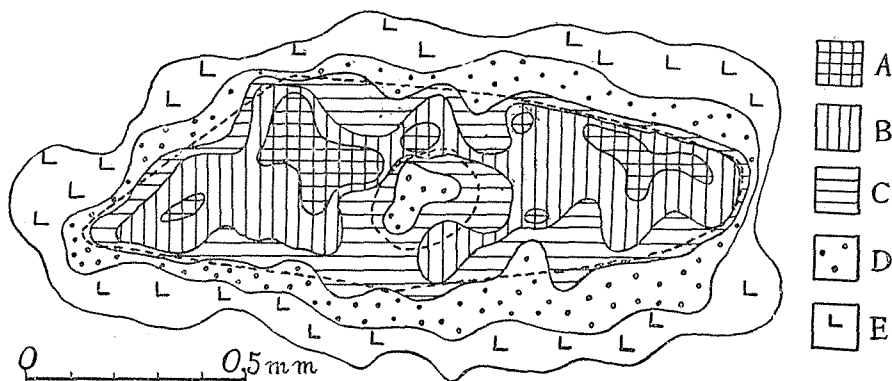
Fig. 1 The alpha track distribution from an allanite of Tanakamiyama granite, Shindenba Quarry. A-over 80 tracks, B-70~30, C-60~70, C-30~60, D-5~30 per 0.01mm 2 for 28 days' exposure.
