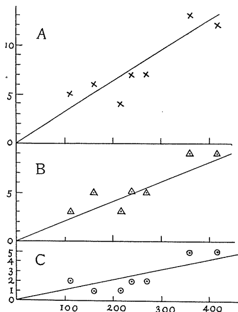
Fig. 3 The relation between the number of long alpha tracks and that of total alpha tracks of some allanites from the Kitashirakawa granite. Ordinate—number of long tracks Abscissa—number of total alpha tracks
