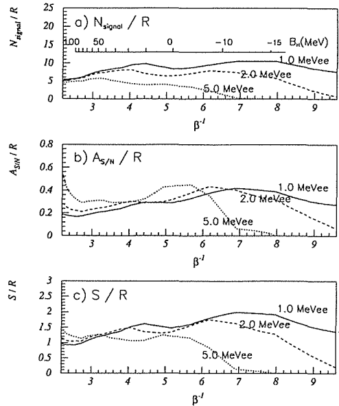
Fig. 23. Expected performance of the signal search with the 1992 data: a) the expected yield of the signal neutrons N_{signal} , b) the ratio of signal to noise A_{S/N} and c) the expected statistical significance of a peak S , normalized by R .
