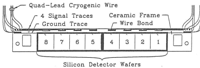
Fig. 8. Schematic layout of a silicon detector unit.
