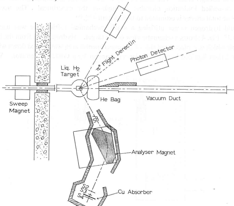
Fig. 3. Schematic diagram of the experimental arrangement for the large angles measurements and the calibration runs.
