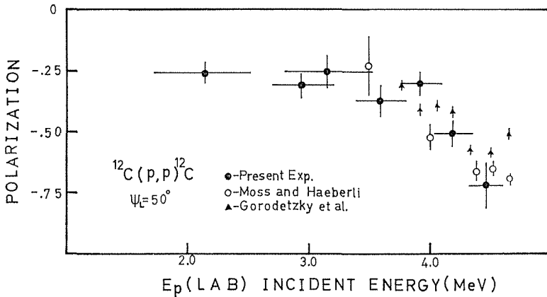
Fig. 2. Absolute polarizations measured at 50^\circ (lab.) compared with other results.
