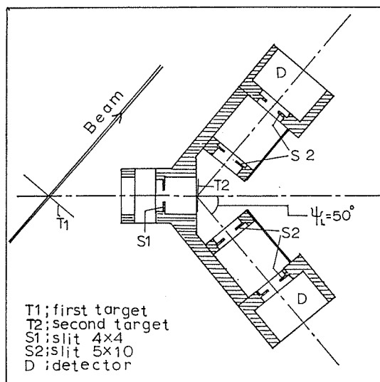
Fig. 1. Schematic drawing of the double scattering apparatus.
