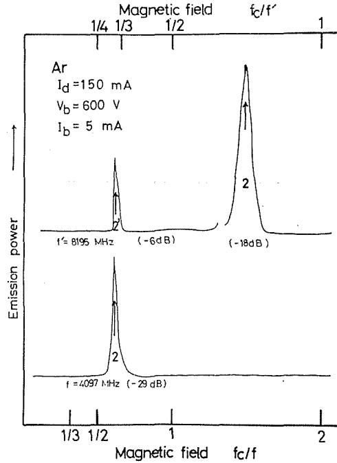
Fig. 9. Emission spectra of the beam-plasma system as a function of the static magnetic field. The lower curve shows the spectrum of f=4,097\text{ MHz} and the upper curve, f'=2f=8,195\text{ MHz} . At the magnetic field where the strongly enhanced emission is seen on the lower curve, the weak emission is also observed on the upper curve. Here, V_b=600\text{ V} , I_b=5\text{ mA} and I_a=150\text{ mA} .
