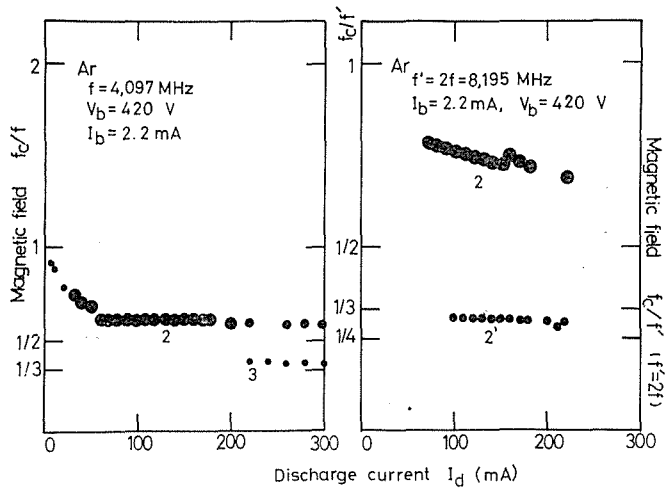
Fig. 10. The magnetic field, f_c/f , where the enhanced emission is observed, is plotted as a function of the discharge current I_a , for the cases of f=4,097 and f'=2f=8,195\text{ MHz} , respectively. Here, V_b=420\text{ V} and I_b=2.2\text{ mA} .
