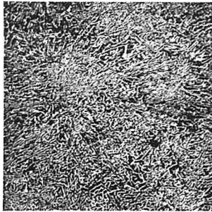
Photo 7. Modified with 0.3% Cd \times 100
