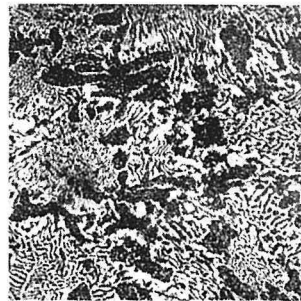
Photo 8. Sn (42%)-Bi alloy. Sand cast \times 100
