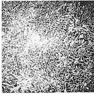
Photo 2. Sb (12.5%)-Pb alloy. Sand cast \times 100
