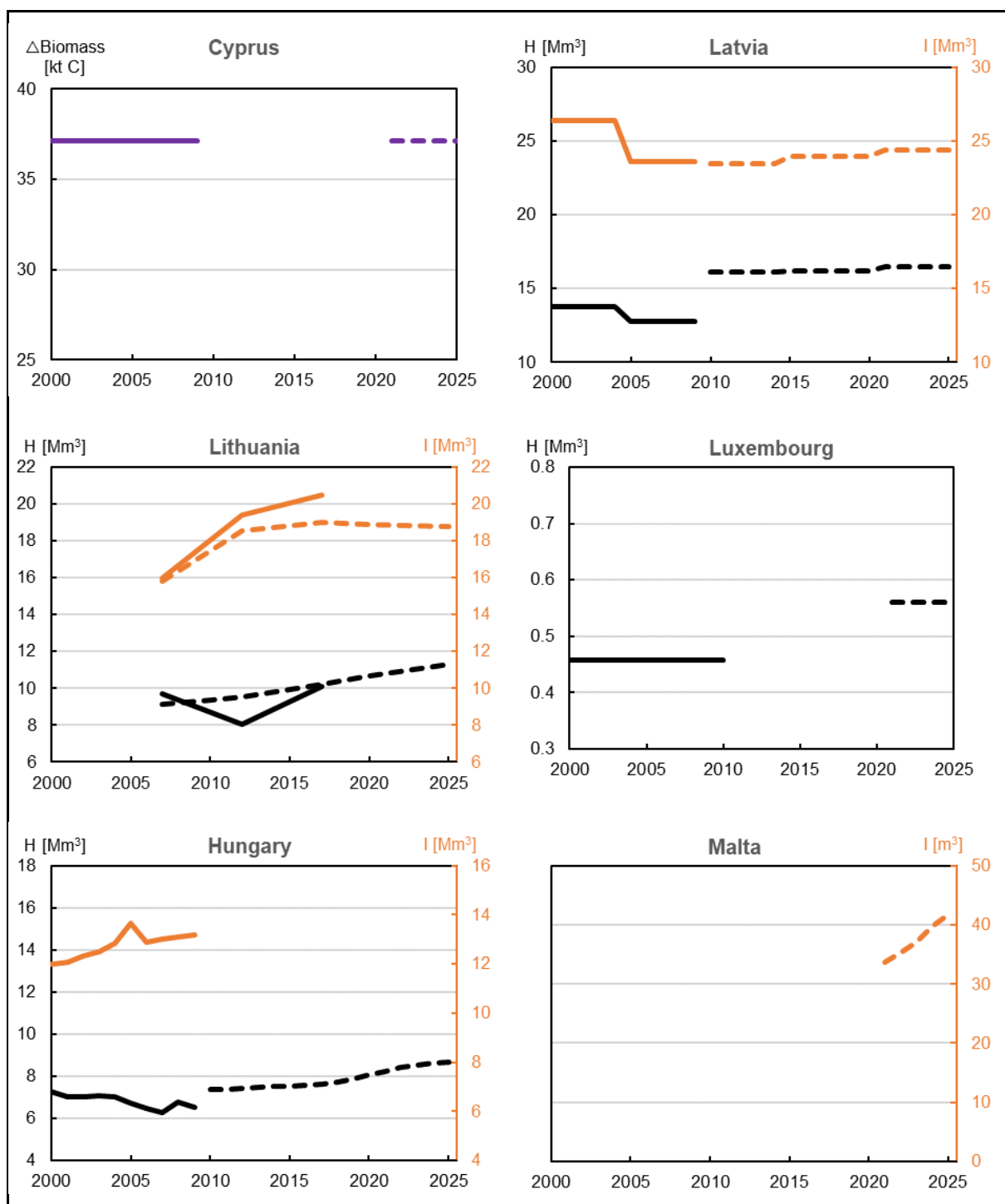
Figure 8 (continued). Cyprus reported biomass change (here shown in purple) instead of harvests or increment. For Malta, no harvests were projected for the FRL. All information shown is based on the NFAPs submitted by the countries.
