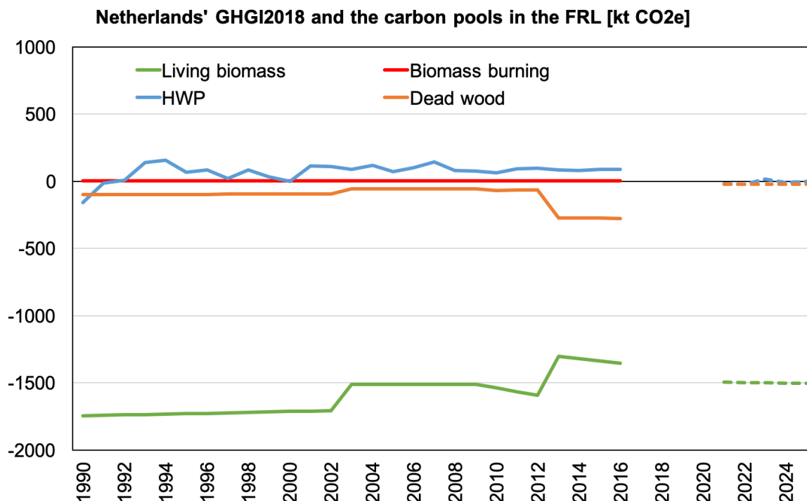
Figure 18. The carbon pools included in the FRL as reported in the GHGI (submission 2018; solid lines), and as projected for the FRL (dashed lines).
