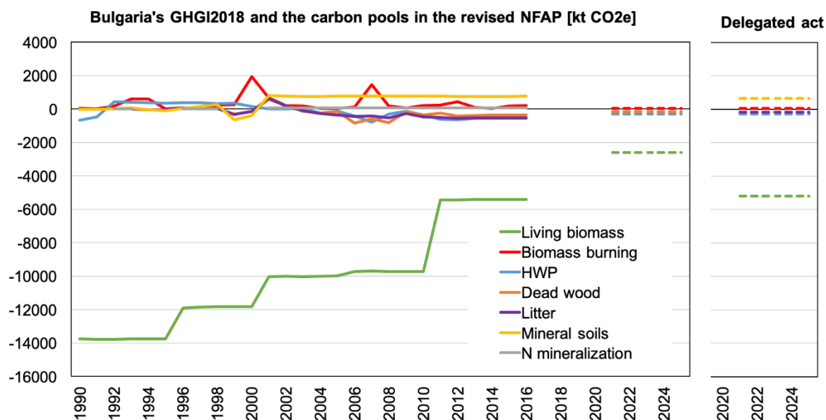
Figure 2. The carbon pools included in the FRL as reported in the GHGI (submission 2018; solid lines), as projected for the FRL in the NFAP (dashed lines, left-hand side), and as included FRL in the delegated act (dashed lines, right-hand side).
