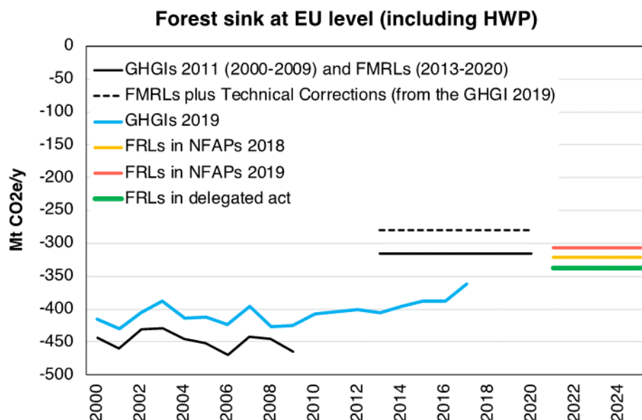
Figure 1. Development of the forest sink at the EU level (sum of all Member States' values), and its relation to the FRLs (according to LULUCF regulation) and to the FMRLs (according to the Kyoto Protocol). The technical corrections added to the FMRLs are from the GHGI 2019 and are not yet the final ones for the period 2013–2020. The FRLs proposed by the Member States in the draft NFAPs in 2018 are shown in yellow, the revised FRLs proposed in the revised NFAPs in 2019 are shown in red, and the FRLs as included in the delegated act are shown in green. The EU values shown include Croatia (not EU Member State when FMRLs were submitted) and the United Kingdom.
