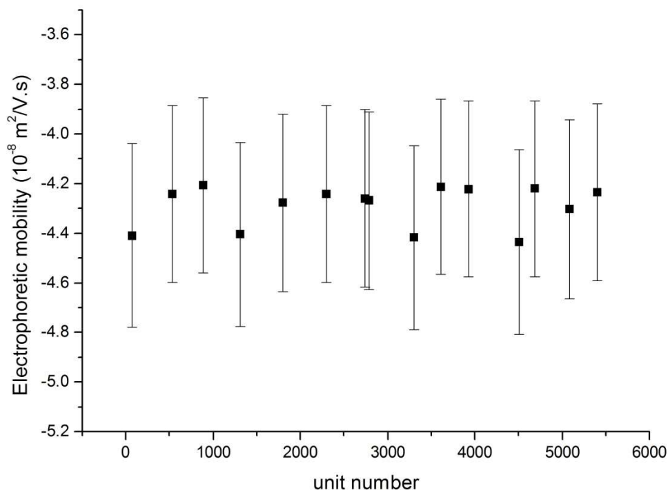
Fig. A Homogeneity data (averages of duplicate results) of ERM-FD305/SRM 1992; electrophoretic mobility by ELS; error bars correspond to the expanded measurement uncertainties ( k = 2 ) for use of the method in repeatability conditions.
