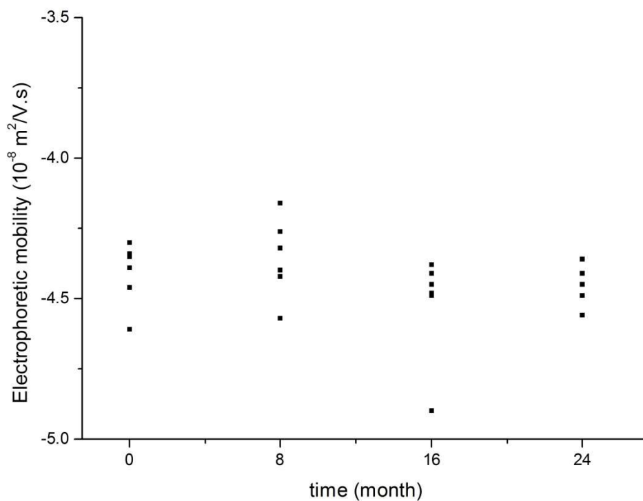
Fig. C Long-term stability data (averages of triplicate results) of ERM-FD305/SRM 1992; electrophoretic mobility by ELS, when stored for several months at 18 °C. Results at time point 0 months correspond to the units that were stored at the reference temperature of 4 °C.
