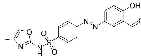
4-((3-Formyl-4-hydroxyphenyl)diazenyl)-N-(4-methyloxazol-2-yl)benzenesulfonamide (FDMB).
