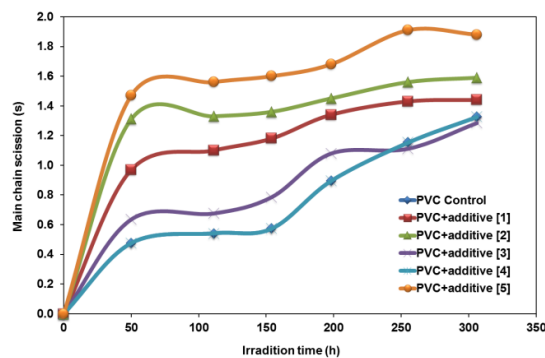
Figure 6. Changes the average number cut per single chain ( S ) during irradiation of PVC films (50 \mu\text{m} ) (control) and with 0.4 wt.% of additives.
