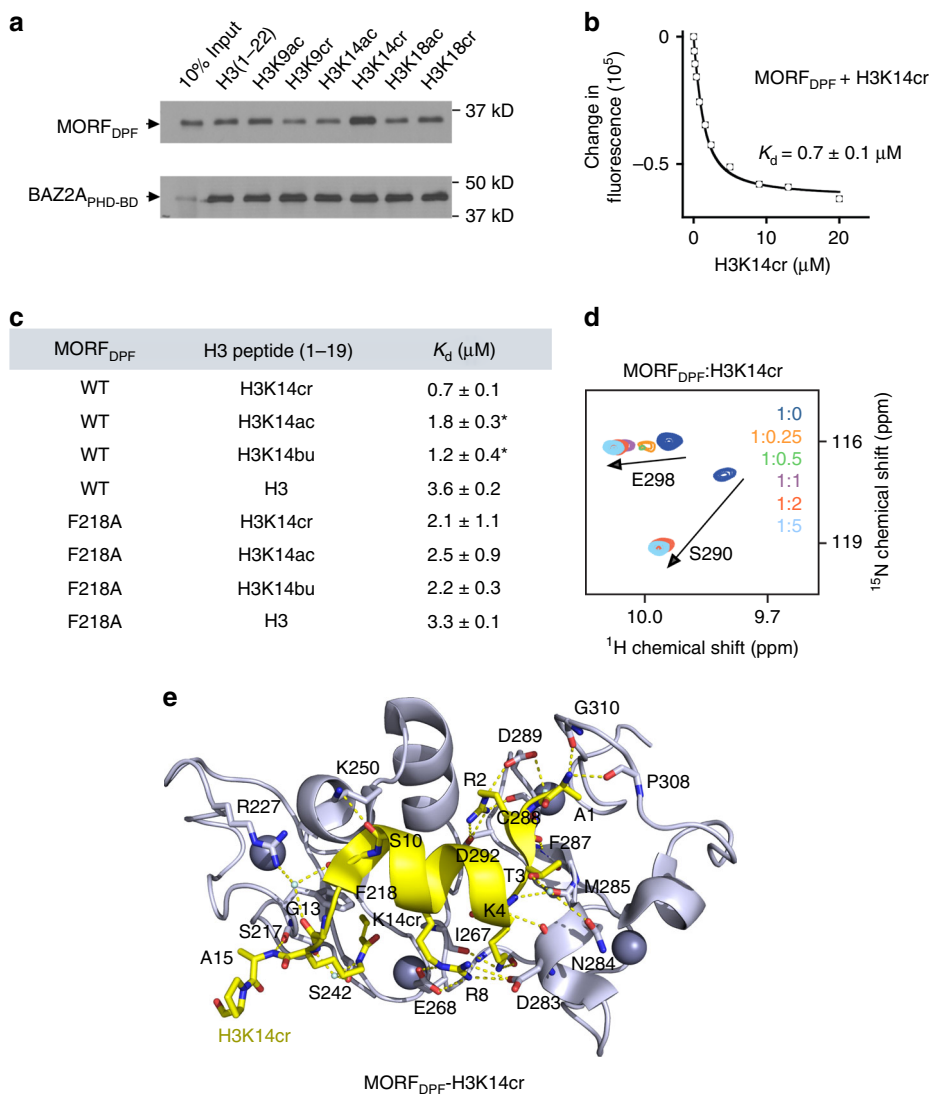
Fig. 2 MORF DPF recognizes H3K14cr. a Western blot analysis of peptide pulldown experiments of GST-MORF DPF with the indicated histone H3 peptides. Peptide pulldowns of the BAZ2A PHD-Bromo domains are shown for comparison. b Representative binding curve used to determine K_d by tryptophan fluorescence. c Binding affinities of MORF DPF to the indicated peptides as measured by tryptophan fluorescence. (*) from 26,27 K_d values were averaged over at least three separate experiments (two for F218A/H3), and error was calculated as standard deviation (SD) between the runs. d Superimposed 1 H, 15 N HSQC spectra of 15 N-labeled MORF DPF , collected as H3K14cr peptide was added stepwise. Spectra are color coded according to the protein:peptide molar ratio (inset). e The ribbon diagram of the MORF DPF -H3K14cr complex structure. H3K14cr peptide is yellow. The histone peptide residues and the residues of MORF DPF involved in the interaction are labeled. Dashed lines indicate hydrogen bonds. Source data are provided as a Source Data file
