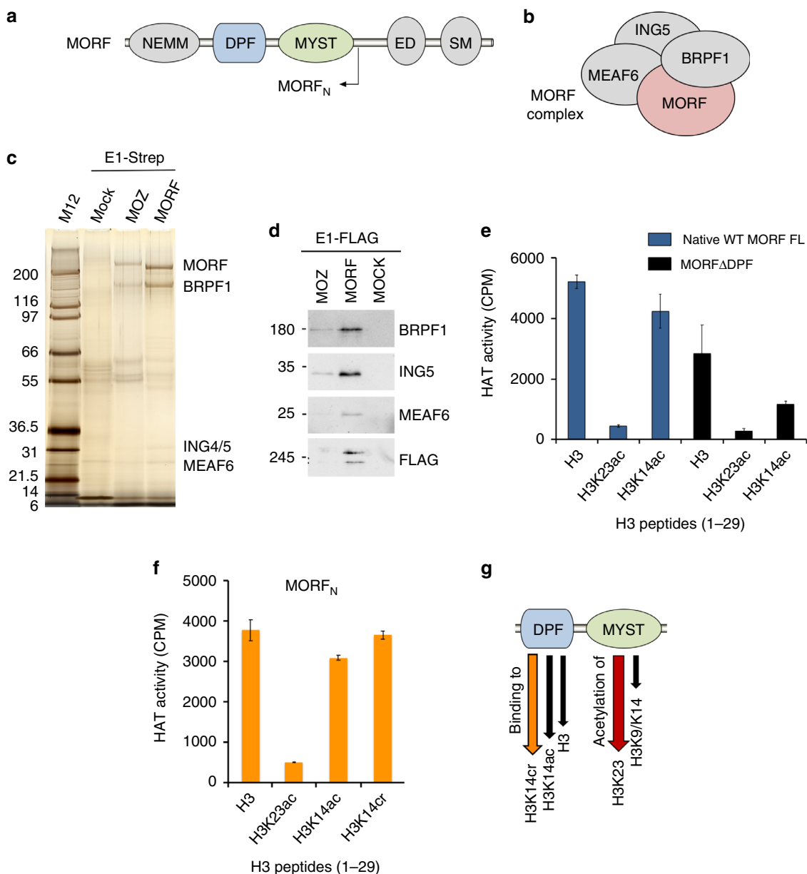
Fig. 1 The native MORF complex is a H3K23-specific HAT. a A diagram of MORF with the MORF N region indicated. b The MORF complex subunit composition. c Purified native MOZ and MORF complexes from K562 cells shown by silver staining. d Confirmation of the subunits of the native purified MORF complex by Western blots using specific antibodies. Source data are provided as a Source Data file. e HAT activity of native MORF complex from K562 cells on the indicated H3 peptides. Liquid HAT assays, in which reactions were spotted on P81 filters and counted by scintillation as counts per minute (CPM). f HAT activity of the MORF N complex overexpressed in 293T cells on indicated H3 peptides. g Cartoon showing interrelated activities of the adjacent DPF and MYST domains. The MYST domain acetylates primarily H3K23 and has some HAT activity on H3K14, whereas MORF DPF binds to unmodified H3 or acylated H3K14, preferring H3K14cr (see below). Error bars indicate the range from duplicate samples, n = 2 independent experiments
