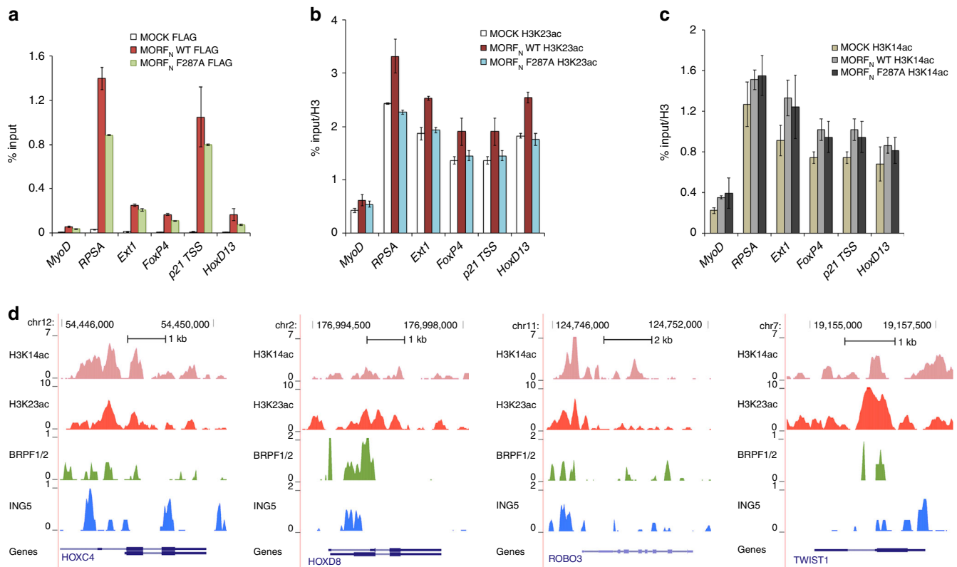
Fig. 6 MORF DPF role in MORF localization in vivo and deposition of H3K23ac. a ChIP analysis of wild-type FLAG-MORF N and mutant FLAG-MORF N F287A in transfected 293T cells. b, c ChIP analysis of H3K23ac ( b ) and H3K14ac ( c ) in the same transfected cells as in a . Acetylation levels were corrected for nucleosomes occupancy (total H3 signal). All ChIP values are based on two independent experiments and error bars indicate the range between the samples. d ChIP-seq profiles of the MORF complex subunits (BRPF1/2 detected with the Brd1 Ab and ING5) in human RKO cells and of histone modifications (H3K14ac and H3K27ac) in HME1 cells are shown. The bottom tracks correspond to the representative RefSeq genes
