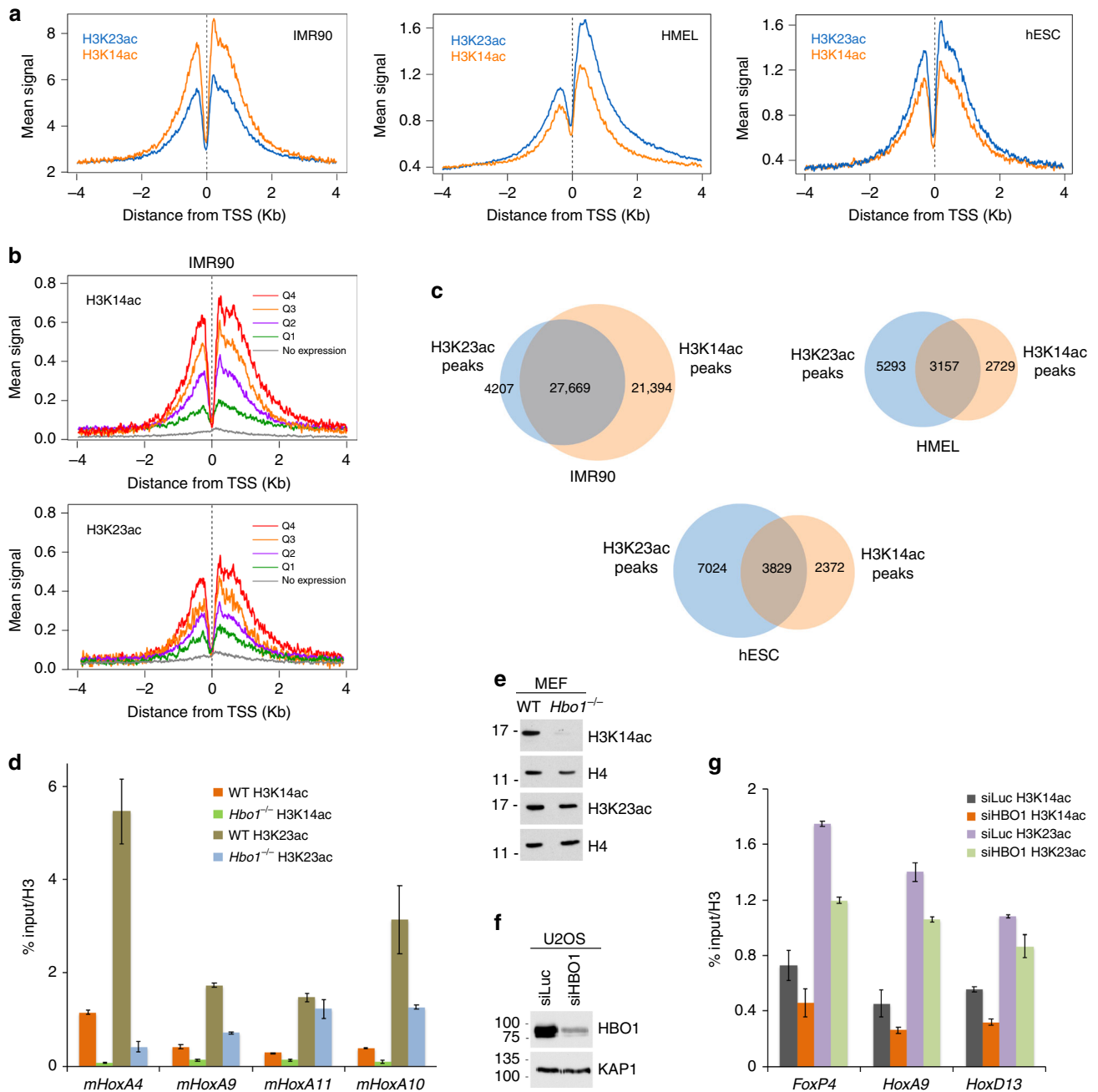
Fig. 7 H3K23ac and H3K14ac colocalization and effect of H3K14ac on H3K23 acetylation at specific genes. a Metagenes analysis of H3K14ac and H3K23ac signals around the transcription start sites of genes observed in ChIP-seq datasets derived from ENCODE in IMR90, hESC and HMEL cells. b RNA-seq analysis of H3K14ac and H3K23ac in IMR90 cell line derived from ENCODE. Genes were subdivided in quartiles corresponding to their expression levels. c Venn diagrams show overlap of the H3K14ac and H3K23ac peaks observed in IMR90, hESC and HMEL cells. d ChIP analysis of H3K23ac and H3K14ac in WT or Hbo1 -/- MEFs. Acetylation levels were corrected for nucleosomes occupancy (total H3 signal). e Western blot analysis of histones purified from WT and Hbo1 -/- MEFs with indicated antibodies. f Western blot analysis of HBO1 and KAP1 in U2OS cells treated with siLuciferase or siHBO1. g ChIP analysis of H3K23ac and H3K14ac in U2OS cells treated with siLuciferase or siHBO1. Acetylation levels were corrected for nucleosomes occupancy (total H3 signal). All ChIP values are based on two independent experiments and error bars in d and g indicate the range from duplicate samples, n = 2 independent experiments. Source data are provided as a Source Data file
