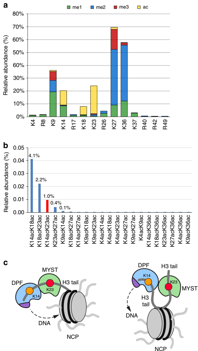
Fig. 8 H3K23ac and H3K14ac co-exist. a Relative abundance of single histone PTMs quantified on the histone H3.2/1 N-terminal tail (residues 1–50). Color coding represents different PTM type, and the y-axis represents the relative abundance; the percentage missing to 100% is the abundance of the unmodified state. b Relative abundance of binary histone PTMs on histone H3. The percentage represents the total relative abundance of histone tails containing the two acetylations listed in the x-axis. The relative abundance of H3K14acK23ac is highlighted in red. c Models for the association of MORF DPF -MYST in cis with a single H3 tail or in trans with two H3 tails of H3K14acyl-NCP
