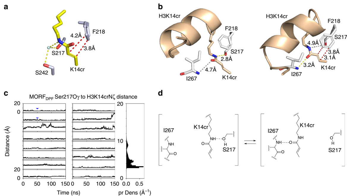
Fig. 3 The ping-pong-like acyllysine-binding mechanism. a A zoom-in view of the H3K14cr-binding pocket of MORF DPPF . Yellow dashed lines represent water (cyan)-mediated hydrogen bonds. Red dashed lines represent short distances indicative of the \pi - \pi interaction. b A close view of the H3K14cr-binding site of the MD generated complex. Yellow and red dashed lines represent hydrogen bonds and short distances indicative of the \pi - \pi interaction, respectively. Gray lines show long distances between the indicated residues. c (left two columns) Time-course of the distance between Ser217O \gamma of MORF DPPF and K14crN \zeta of H3. Blue triangles correspond to the timing of snapshots shown in b . All plots share the same ordinate (between 0 and 20 Å). (Right column) Distribution of the distance between two atoms. Abscissa and ordinate represent the probability density (pr Dens) and the distance between Ser217O \gamma of MORF DPPF and K14crN \zeta of H3. d A schematic showing shuffling of K14cr between two conformations in the MORF DPPF -H3K14cr complex
