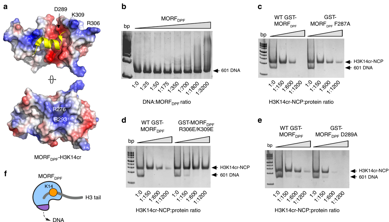
Fig. 5 MORF DPF has DNA-binding activity. a Electrostatic surface potential of the MORF DPF in complex with H3K14cr is shown. Blue and red colors indicate positive and negative charges, respectively. b EMSA of 147-bp 601 DNA incubated with increasing amounts of WT MORF DPF . DNA to protein molar ratio is shown below the gel image. c–e EMSA of H3K14cr-NCP incubated with increasing amounts of WT or mutant GST-MORF DPF . H3K14cr-NCP to protein molar ratio is shown below each gel image. f A schematic showing the dual interaction of MORF DPF with histone tail and DNA
