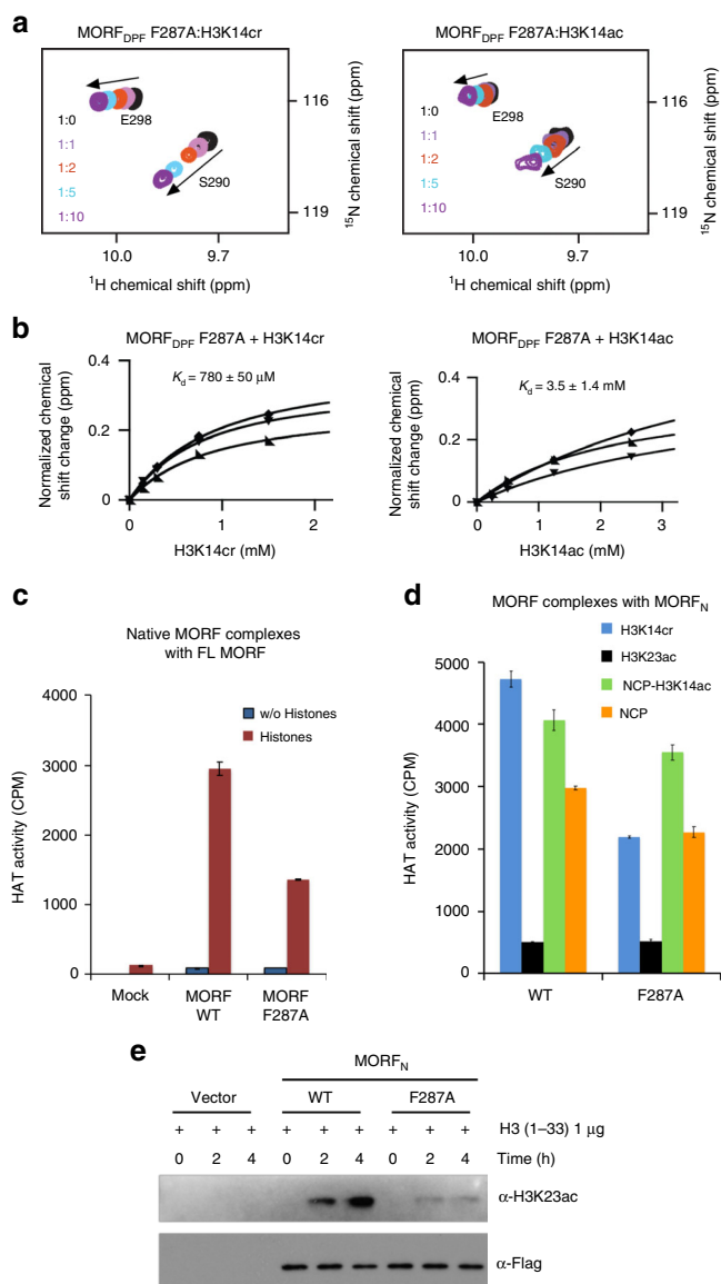
Fig. 4 H3K23 acetylation depends on functional MORF DPF . a Superimposed 1 H, 15 N HSQC spectra of MORF DPF F287A mutant collected as indicated peptides were added stepwise. Spectra are color coded according to the protein:peptide molar ratio (inset). b Representative binding curves used to determine K_d s for the interactions of MORF DPF F287A with indicated peptides by NMR. Error was calculated as SD. c HAT activity of native MORF wild-type and F287A mutant complexes from K562 cells on native free core histones. Liquid HAT assays, in which reactions were spotted on P81 filters and counted by scintillation as counts per minute (CPM). d HAT activities of wild-type and mutated MORF N complexes purified from 293T cells using indicated H3 peptides (residues 1–29) or recombinant unmodified nucleosomes (NCP) or nucleosomes containing H3K14ac (H3K14ac-NCP) as substrates. Error bars in c and d indicate the range from duplicate samples, n = 2 independent experiments. e Western blot analysis of HAT assays with purified overexpressed wild-type and mutant MORF N using H3 peptide (residues 1–33) as substrate
