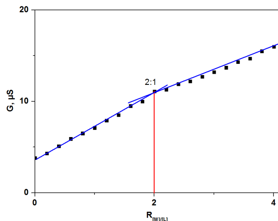
Figure 2. Conductometric titration in the case of ligand 3 with Sm 3+ (C L = 3.8 × 10 -5 mol/L) in methanol.
