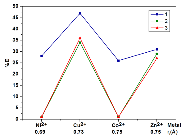
Figure 3. Trends of the extraction percentages (%E) for some salt metal picrates from water into dichloromethane.
