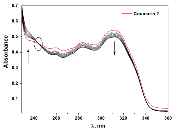
Figure 1. UV absorption spectra of complexation of Sm 3+ by compound 2 in methanol, C_L = 5 \times 10^{-5} M, 0 \leq R_{M/L} \leq 5 , at 25 °C.
