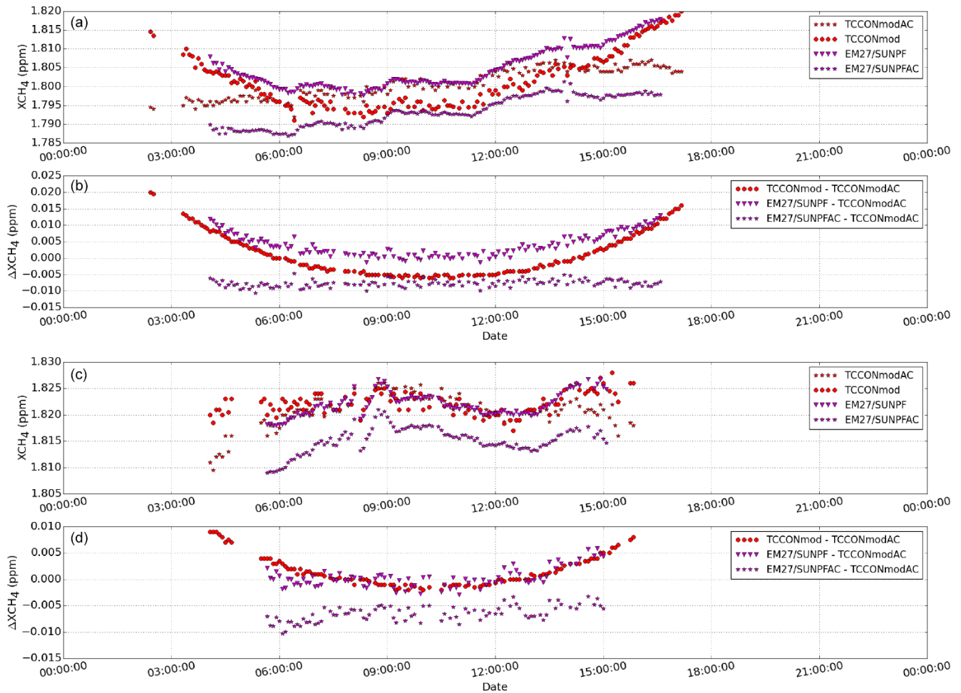
Figure 5. (a) XCH_4 plotted for TCCONmod and EM27/SUN retrievals with the TCCON a priori and with a modified a priori (calculated using in situ, AirCore, and TCCON map files; labelled with AC at the end) for measurements performed on 15 May 2017 at Sodankylä. Panel (b) shows the difference between the two retrievals in absolute units. Panels (c) and (d) show the same plots as mentioned above for measurements performed on 28 August 2017 at Sodankylä.
