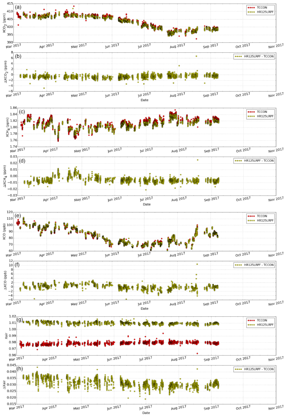
Figure C1. Time series of X_{CO_2} (a), X_{CH_4} (c), X_{CO} (e), and X_{air} (g) retrievals for TCCON and HR125LR using the standard procedure with the TCCON a priori for measurements performed at Sodankylä in 2017. The difference of X_{CO_2} (b), X_{CH_4} (d), X_{CO} (f), and X_{air} (h) time series for HR125LR relative to the reference TCCON results.
