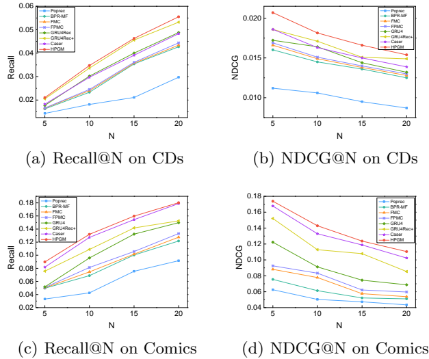
Fig. 2. Ranking performance(NDCG and Recall) with baselines on Amazon-CDs and GoodReads-Comics.
