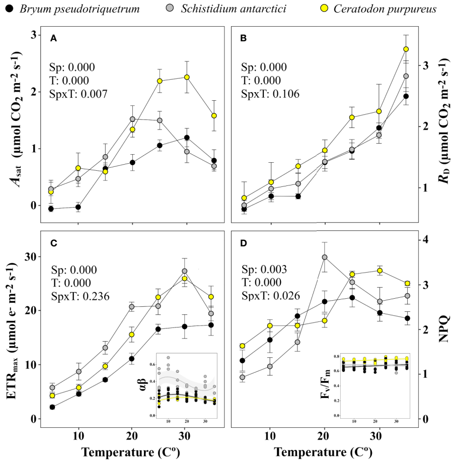
FIGURE 7 | Temperature response curve of three East Antarctic moss species for (A) saturating net CO 2 assimilation ( A_{sat} ), (B) dark respiration ( R_D ), (C) maximum electron transport rate ( ETR_{max} ), and (D) non-photochemical quenching (NPQ). Inset graph of (C) shows variation in the product of absorbance and partitioning of photons ( \alpha\beta ) used for calculation of ETR across temperature ( R^2 = 0.068, 0.063, \text{ and } 0.095 for C. purpureus , S. antarctici , and B. pseudotriquetrum , respectively). Inset graph of (D) shows stability of F_v/F_m across temperature ( R^2 = 0.086, 0.028 \text{ and } 0.046 for C. purpureus , S. antarctici and B. pseudotriquetrum , respectively). P values results from two-way ANOVA are shown in the upper-left corner of each graph. Mean \pm se ( n = 4-6 , except for the light curve derived parameter \alpha\beta , where n = 3-5 ).
