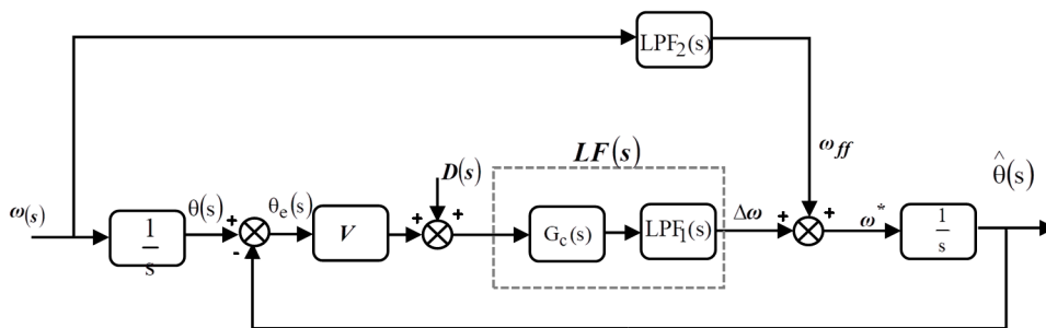
Figure 3. Small signal model of FPLL.
