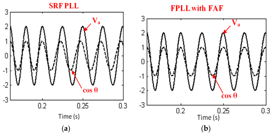
Figure 7. Response for frequency changeover from 50 to 40 Hz: (a) \cos \theta of SRF PLL, (b) \cos \theta of FPLL with frequency adaptive filter output.
