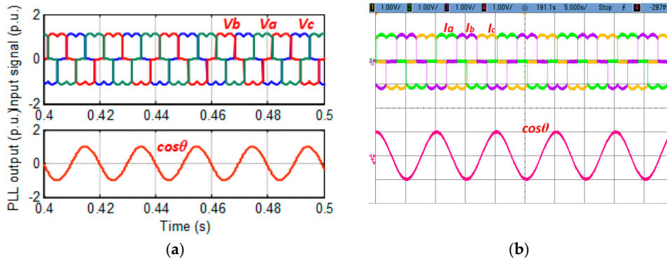
Figure 11. The response of adaptive FPLL under harmonic input: (a) Simulation response for 5th and 7th order harmonic input and (b) experimental results for 5th and 7th order harmonic input.
