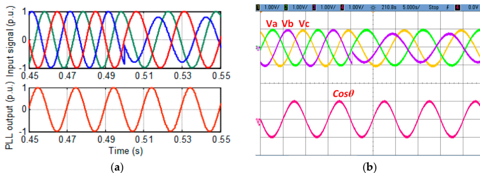
Figure 10. The response of adaptive FPLL: (a) Simulation response under 30^\circ , phase shift and (b) experimental results under 30^\circ phase shift.
