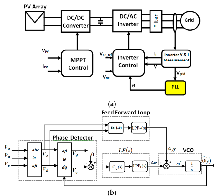
Figure 1. Grid-connected photovoltaic system (a) basic block diagram, (b) structure of phase-locked loop (PLL).
