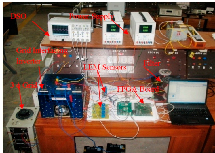
Figure 6. Prototype of proposed PLL.
