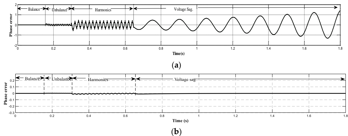
Figure 13. System phase error, (a) conventional PLL [20], (b) adaptive feed-forward PLL.
