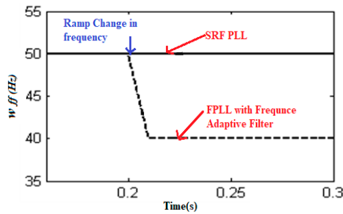
Figure 8. Feed-forward frequency under frequency deviation.
