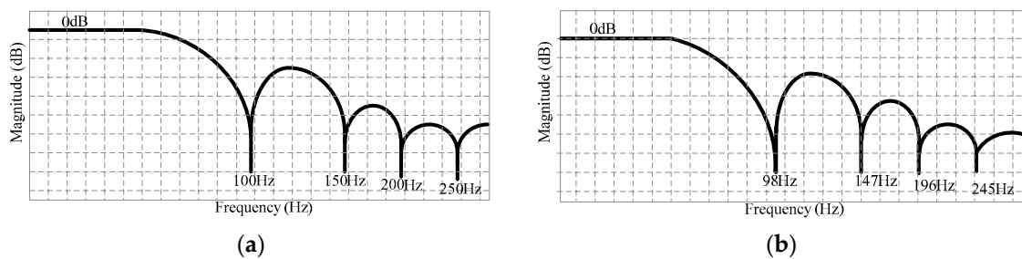
Figure 5. Filtering characteristics of PLLs. (a) Conventional FPLL [20], (b) proposed adaptive feed-forward PLL.
