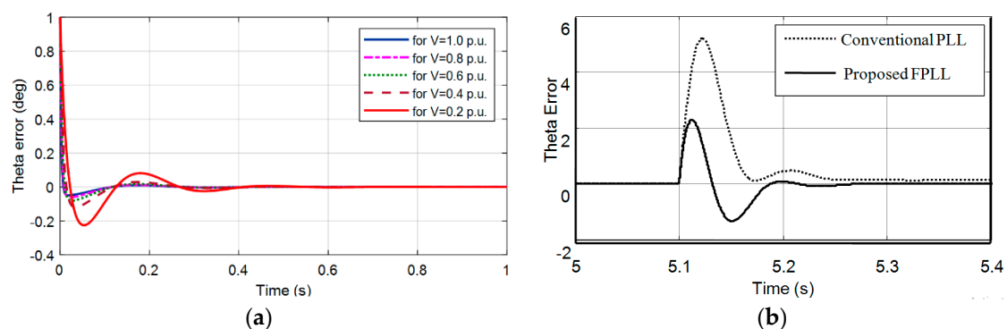
Figure 4. Theta Error (a) for a change in input voltage, (b) for step change in frequency.
