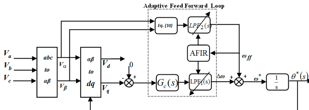
Figure 2. Structure of adaptive feed-forward frequency phase-locked loop (FPLL).
