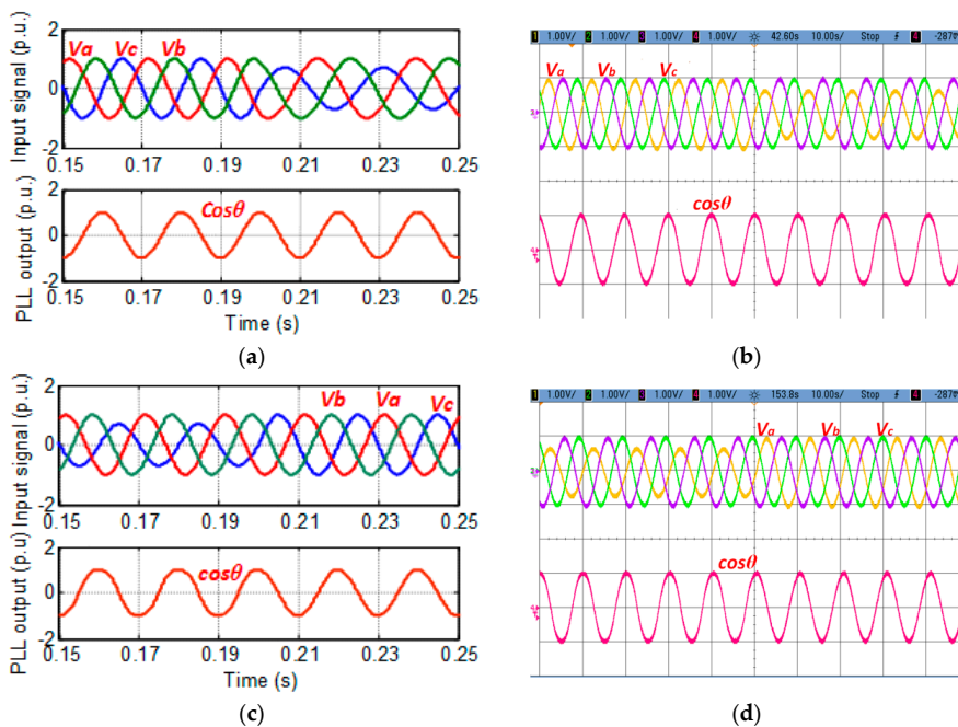
Figure 12. Response of PLL under unbalanced condition: (a) 3-φ balanced input to 3-φ unbalanced input (simulation), (b) 3-φ balanced input to 3-φ unbalanced input (experimental), (c) 3-φ unbalanced input to 3-φ balanced input (simulation), and (d) 3-φ unbalanced input to 3-φ balanced input (experimental).
