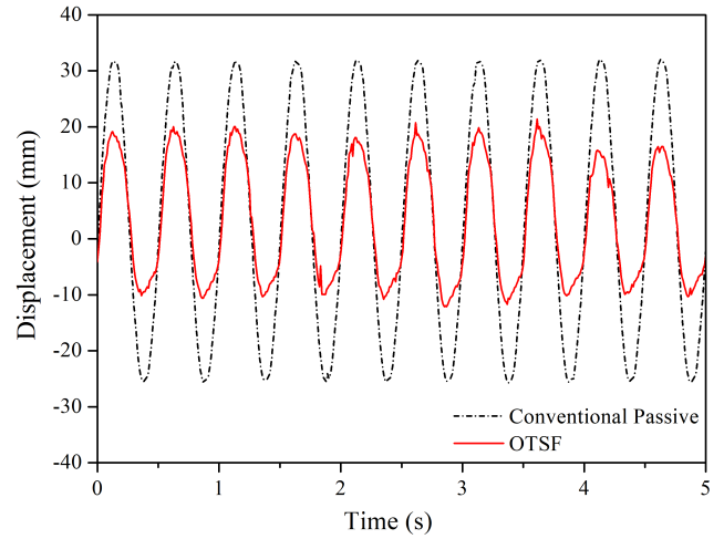
FIGURE 8. Suspension displacement under 2 Hz sinusoidal excitation.
